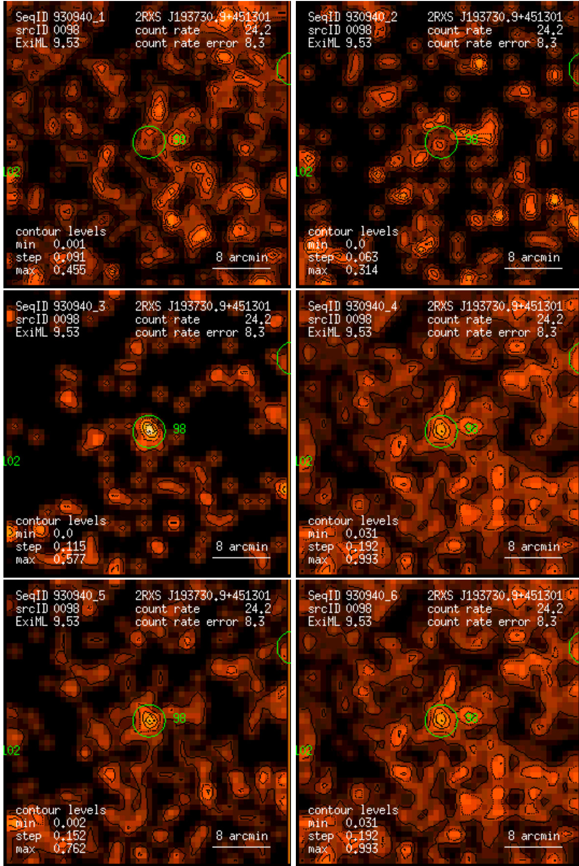
Figure 98: RASS 930940: detection 0098: band rate images, Gaussian filter: (1) PSPC channels 11 – 41, (2) 52 – 90, (3) 91 – 201, (4) 11 – 235, (5) 52 – 201, (6) 11 – 201. Broad band rates in counts/ks. Band rate contour levels in counts/ks/arcmin 2 .
