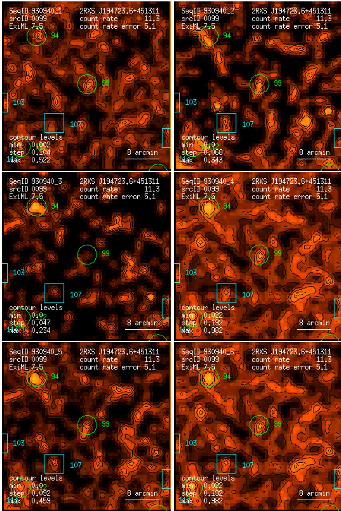
Figure 99: RASS 930940: detection 0099: band rate images, Gaussian filter: (1) PSPC channels 11 – 41, (2) 52 – 90, (3) 91 – 201, (4) 11 – 235, (5) 52 – 201, (6) 11 – 201. Broad band rates in counts/ks. Band rate contour levels in counts/ks/arcmin 2 .
