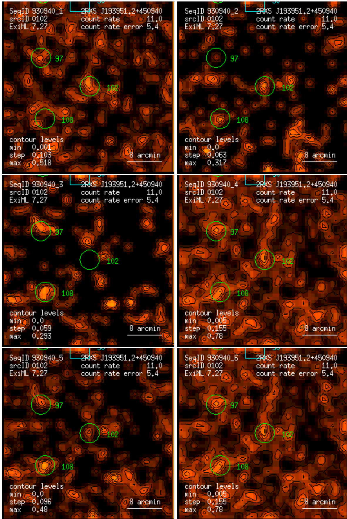
Figure 102: RASS 930940: detection 0102: band rate images, Gaussian filter: (1) PSPC channels 11 – 41, (2) 52 – 90, (3) 91 – 201, (4) 11 – 235, (5) 52 – 201, (6) 11 – 201. Broad band rates in counts/ks. Band rate contour levels in counts/ks/arcmin 2 .
