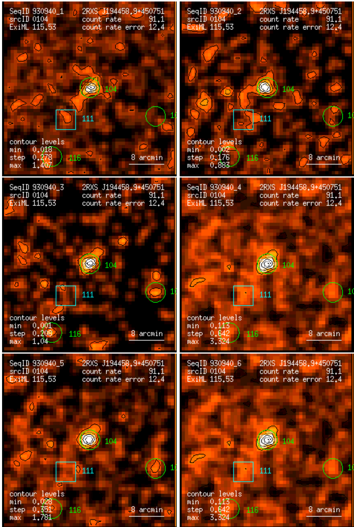
Figure 104: RASS 930940: detection 0104: band rate images, Gaussian filter: (1) PSPC channels 11 – 41, (2) 52 – 90, (3) 91 – 201, (4) 11 – 235, (5) 52 – 201, (6) 11 – 201. Broad band rates in counts/ks. Band rate contour levels in counts/ks/arcmin 2 .
