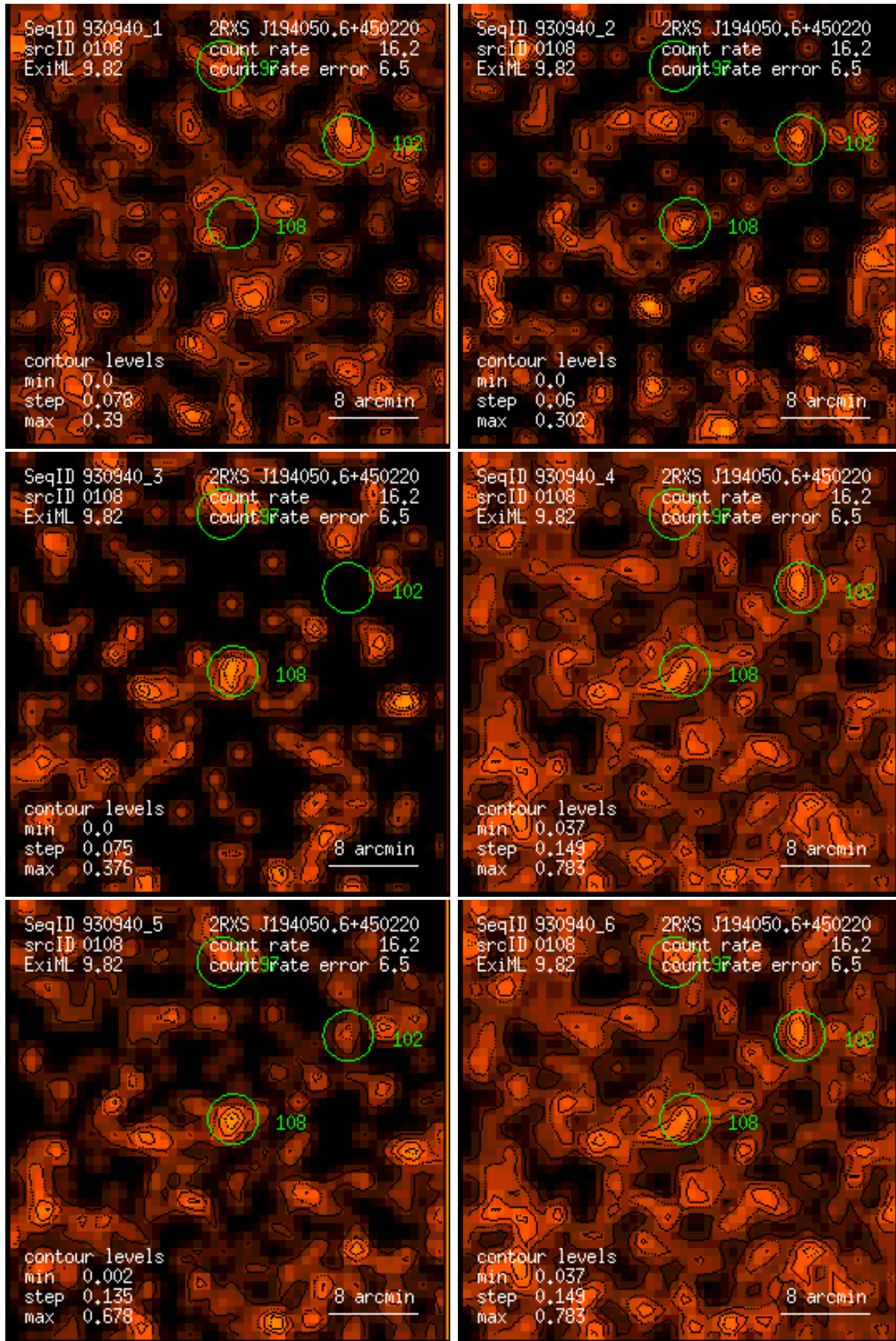
Figure 108: RASS 930940: detection 0108: band rate images, Gaussian filter: (1) PSPC channels 11 – 41, (2) 52 – 90, (3) 91 – 201, (4) 11 – 235, (5) 52 – 201, (6) 11 – 201. Broad band rates in counts/ks. Band rate contour levels in counts/ks/arcmin 2 .
