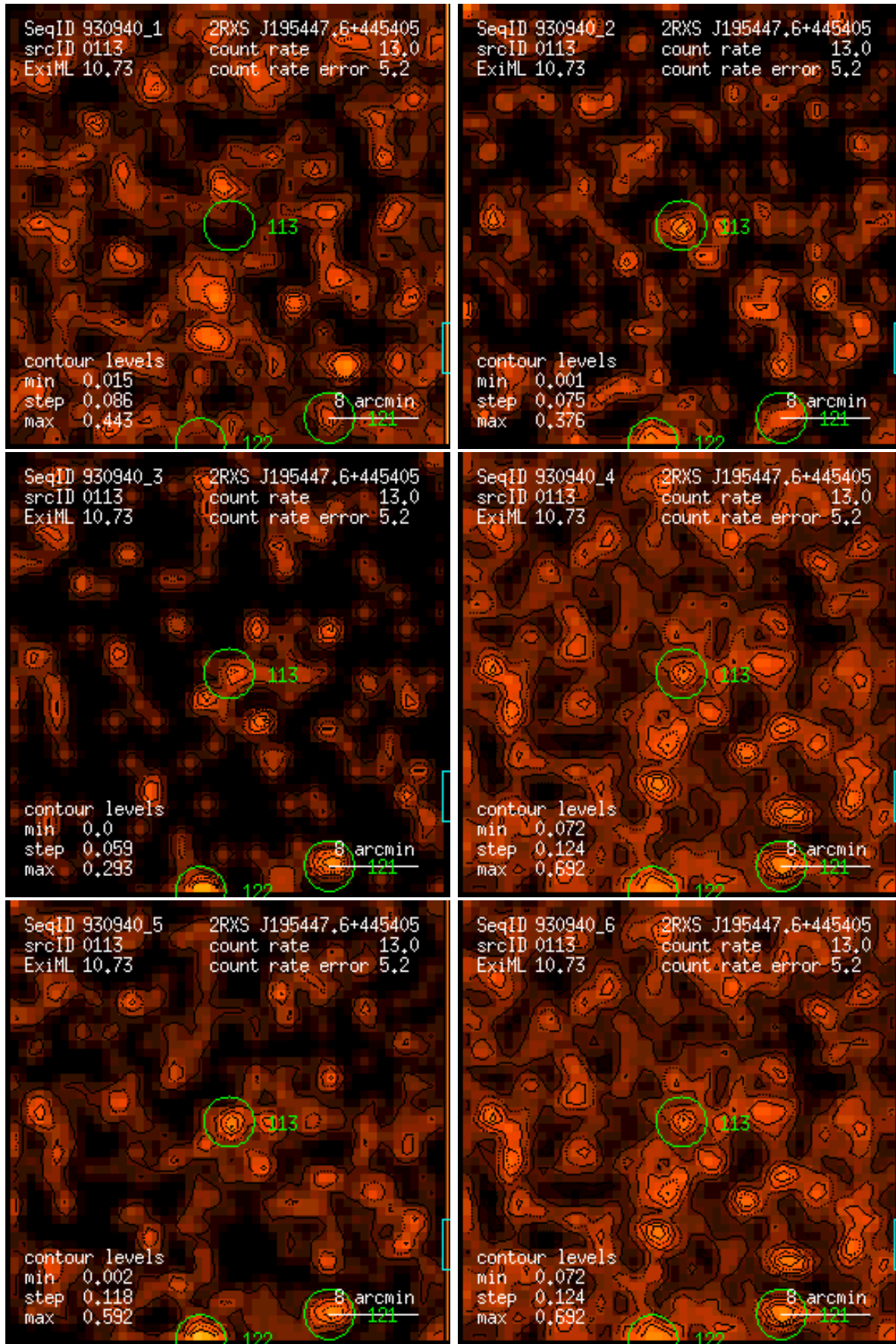
Figure 113: RASS 930940: detection 0113: band rate images, Gaussian filter: (1) PSPC channels 11 – 41, (2) 52 – 90, (3) 91 – 201, (4) 11 – 235, (5) 52 – 201, (6) 11 – 201. Broad band rates in counts/ks. Band rate contour levels in counts/ks/arcmin 2 .
