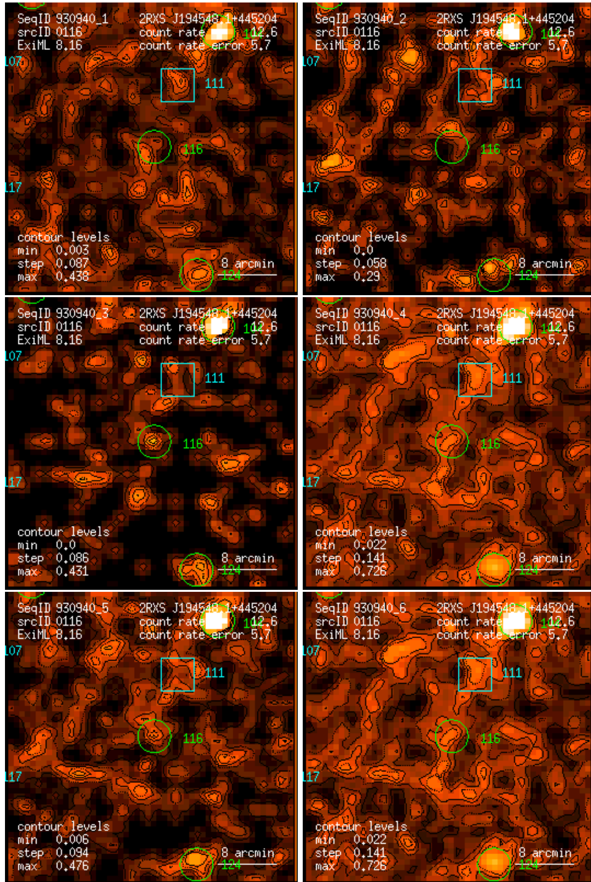
Figure 116: RASS 930940: detection 0116: band rate images, Gaussian filter: (1) PSPC channels 11 – 41, (2) 52 – 90, (3) 91 – 201, (4) 11 – 235, (5) 52 – 201, (6) 11 – 201. Broad band rates in counts/ks. Band rate contour levels in counts/ks/arcmin 2 .
