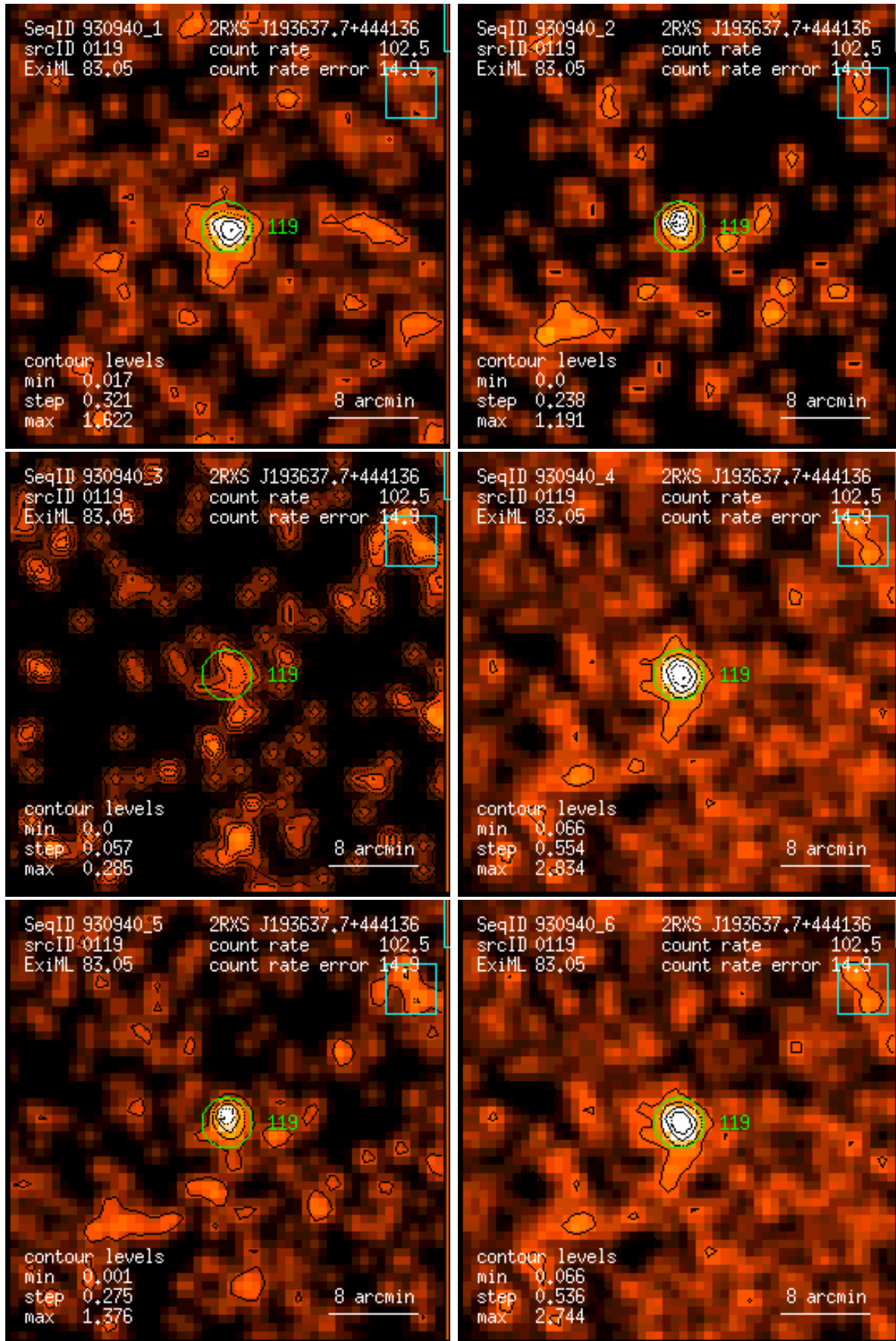
Figure 119: RASS 930940: detection 0119: band rate images, Gaussian filter: (1) PSPC channels 11 – 41, (2) 52 – 90, (3) 91 – 201, (4) 11 – 235, (5) 52 – 201, (6) 11 – 201. Broad band rates in counts/ks. Band rate contour levels in counts/ks/arcmin 2 .
