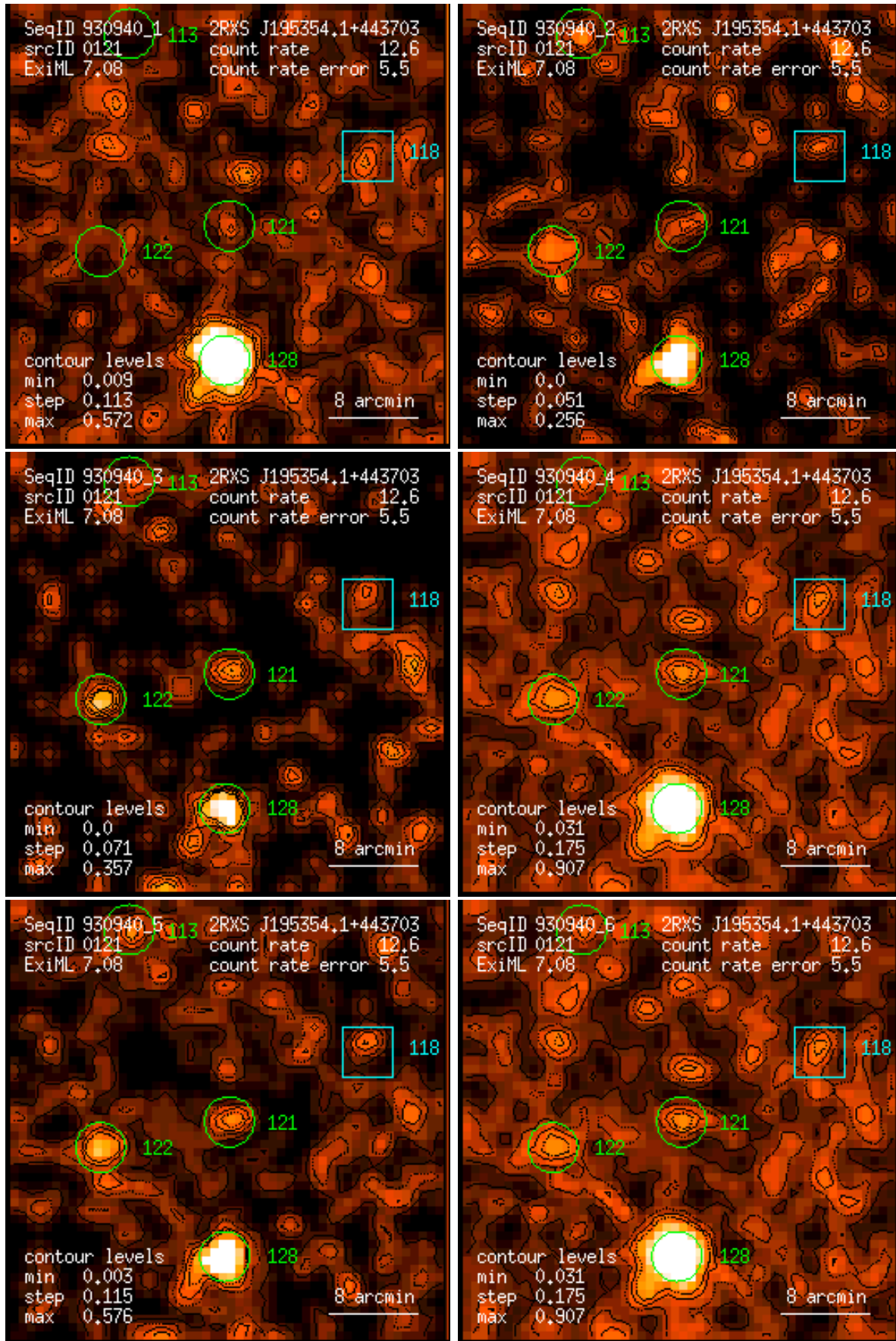
Figure 121: RASS 930940: detection 0121: band rate images, Gaussian filter: (1) PSPC channels 11 – 41, (2) 52 – 90, (3) 91 – 201, (4) 11 – 235, (5) 52 – 201, (6) 11 – 201. Broad band rates in counts/ks. Band rate contour levels in counts/ks/arcmin 2 .
