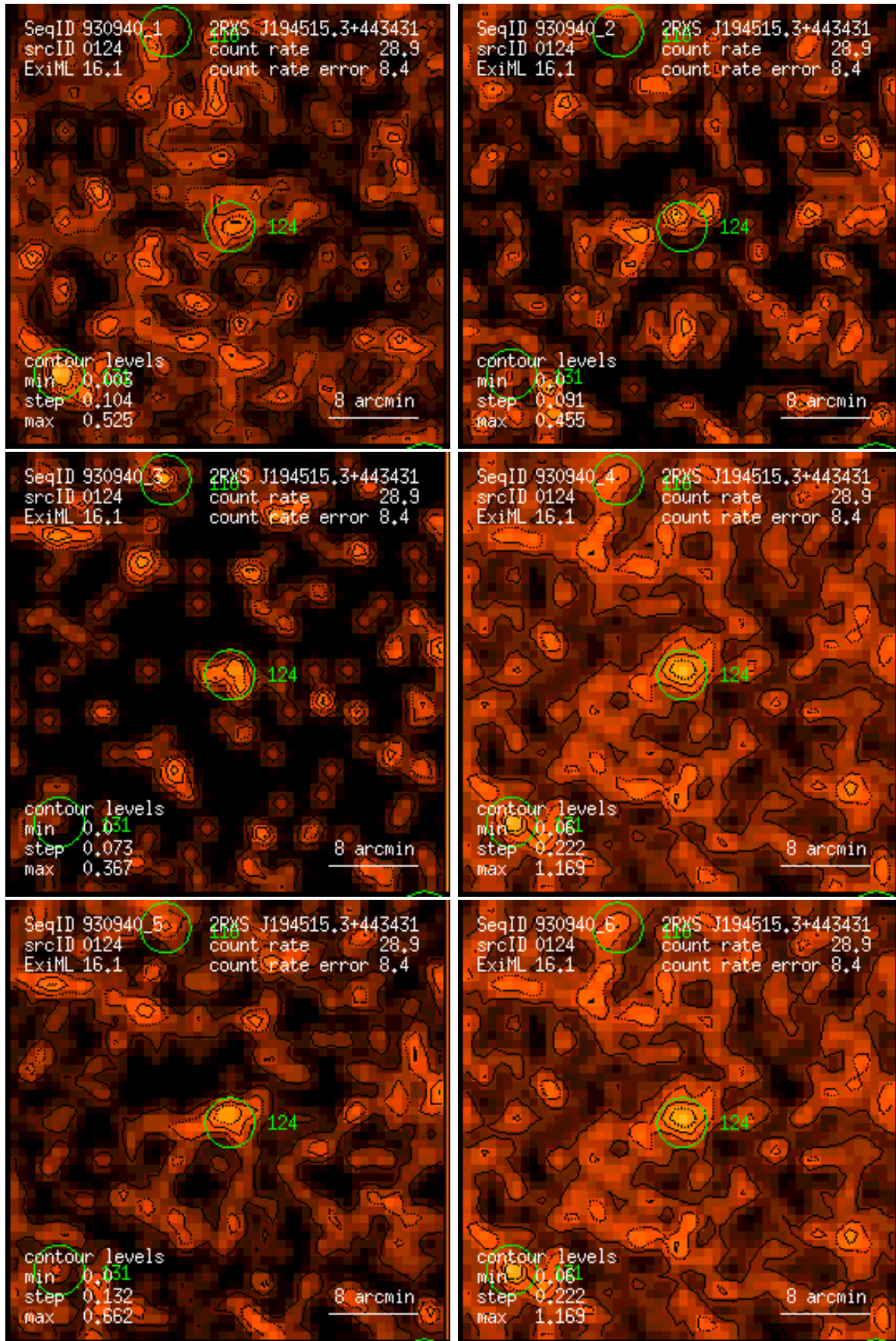
Figure 124: RASS 930940: detection 0124: band rate images, Gaussian filter: (1) PSPC channels 11 – 41, (2) 52 – 90, (3) 91 – 201, (4) 11 – 235, (5) 52 – 201, (6) 11 – 201. Broad band rates in counts/ks. Band rate contour levels in counts/ks/arcmin 2 .
