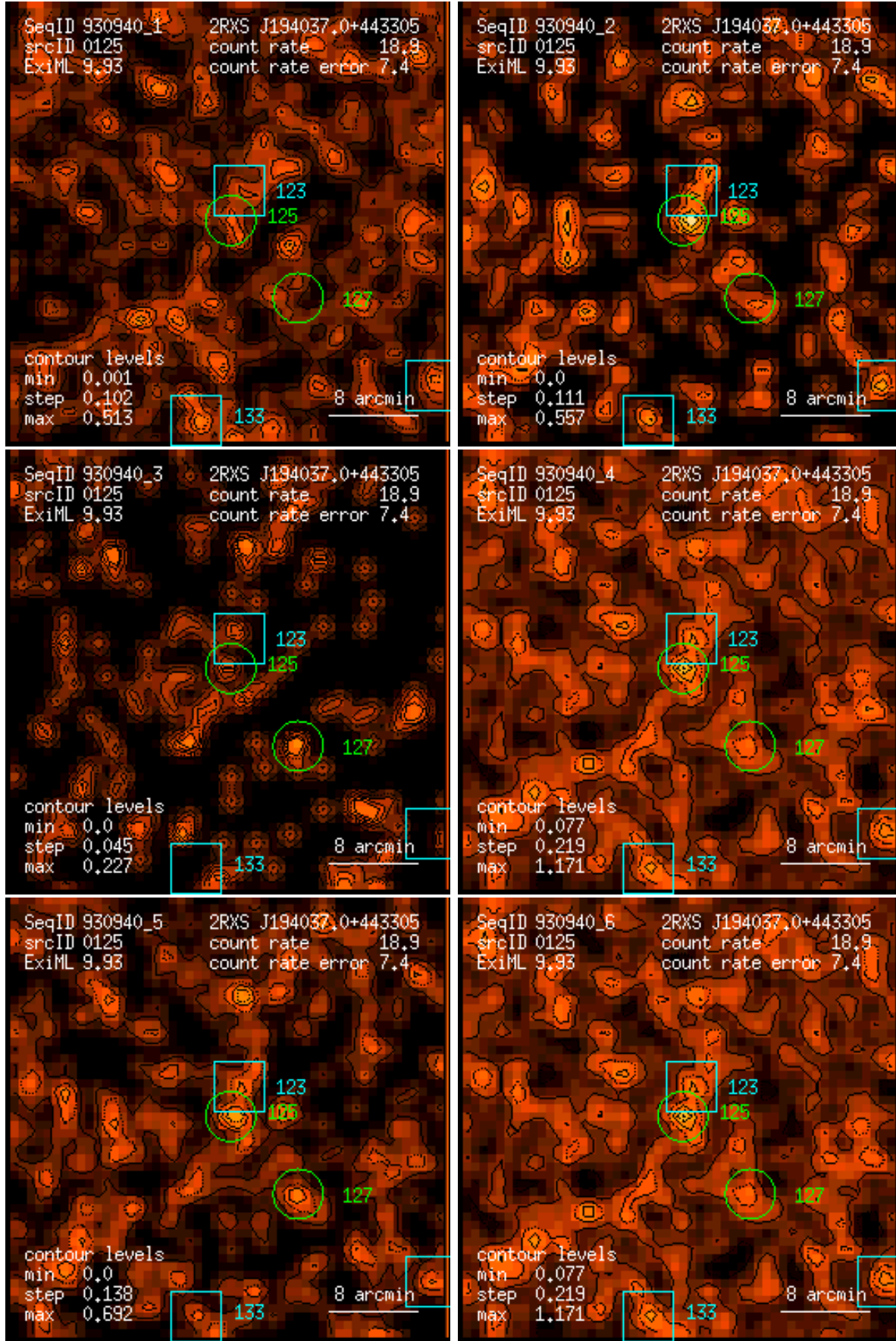
Figure 125: RASS 930940: detection 0125: band rate images, Gaussian filter: (1) PSPC channels 11 – 41, (2) 52 – 90, (3) 91 – 201, (4) 11 – 235, (5) 52 – 201, (6) 11 – 201. Broad band rates in counts/ks. Band rate contour levels in counts/ks/arcmin 2 .
