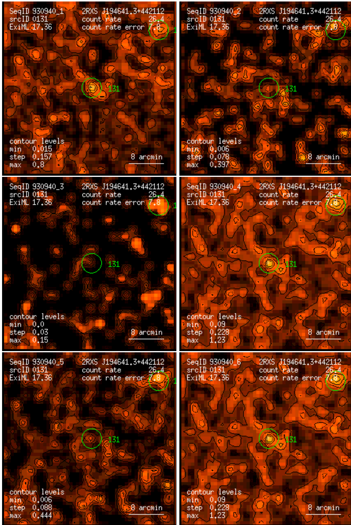
Figure 131: RASS 930940: detection 0131: band rate images, Gaussian filter: (1) PSPC channels 11 – 41, (2) 52 – 90, (3) 91 – 201, (4) 11 – 235, (5) 52 – 201, (6) 11 – 201. Broad band rates in counts/ks. Band rate contour levels in counts/ks/arcmin 2 .
