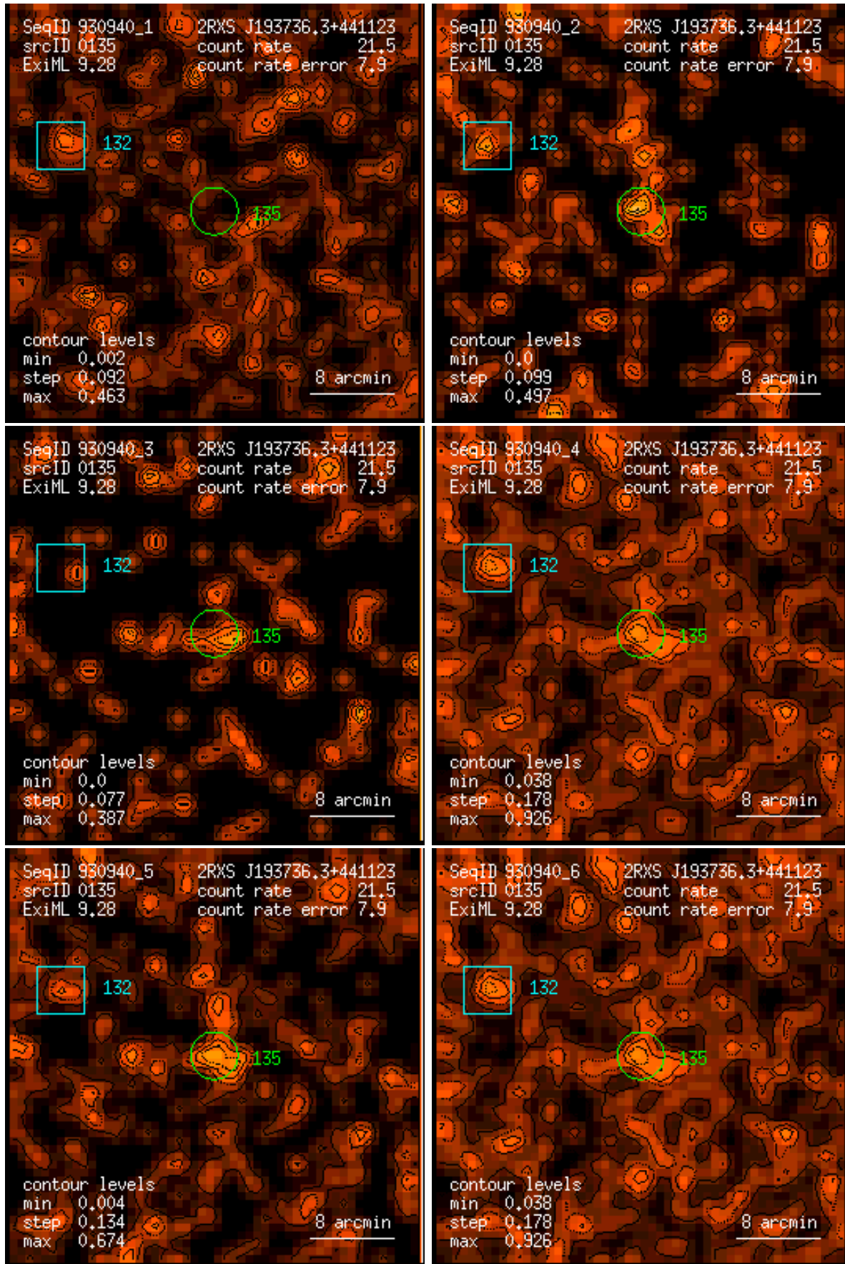
Figure 135: RASS 930940: detection 0135: band rate images, Gaussian filter: (1) PSPC channels 11 – 41, (2) 52 – 90, (3) 91 – 201, (4) 11 – 235, (5) 52 – 201, (6) 11 – 201. Broad band rates in counts/ks. Band rate contour levels in counts/ks/arcmin 2 .
