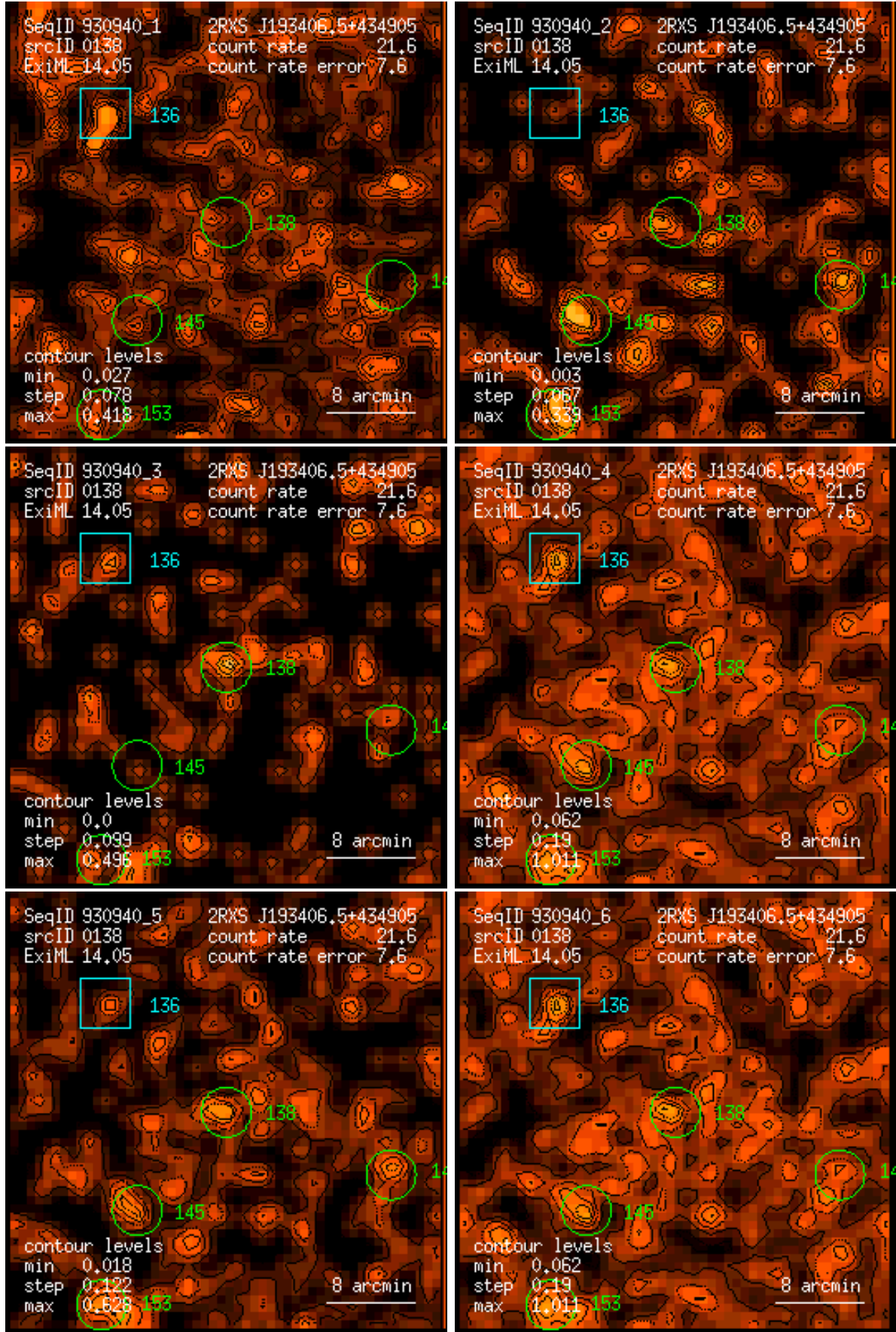
Figure 138: RASS 930940: detection 0138: band rate images, Gaussian filter: (1) PSPC channels 11 – 41, (2) 52 – 90, (3) 91 – 201, (4) 11 – 235, (5) 52 – 201, (6) 11 – 201. Broad band rates in counts/ks. Band rate contour levels in counts/ks/arcmin 2 .
