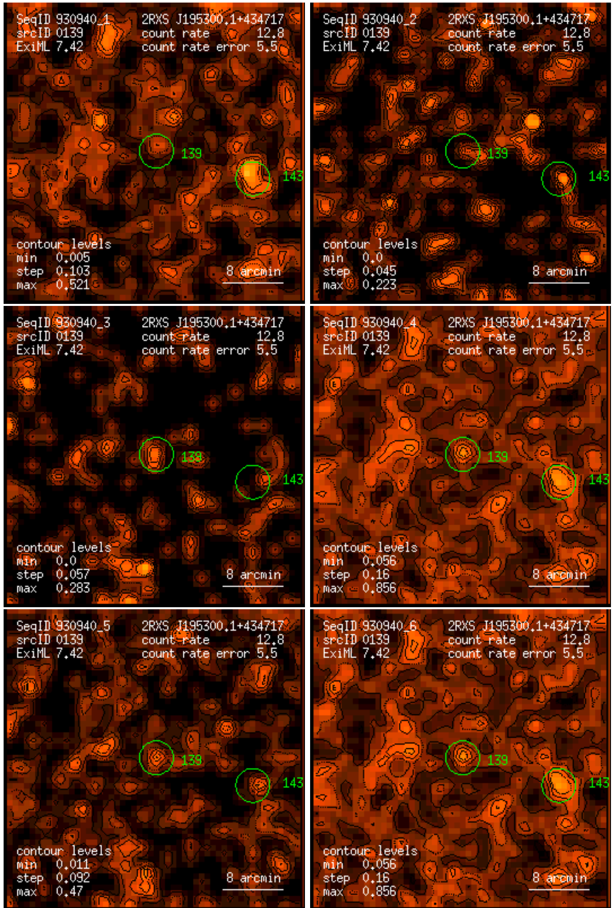
Figure 139: RASS 930940: detection 0139: band rate images, Gaussian filter: (1) PSPC channels 11 – 41, (2) 52 – 90, (3) 91 – 201, (4) 11 – 235, (5) 52 – 201, (6) 11 – 201. Broad band rates in counts/ks. Band rate contour levels in counts/ks/arcmin 2 .
