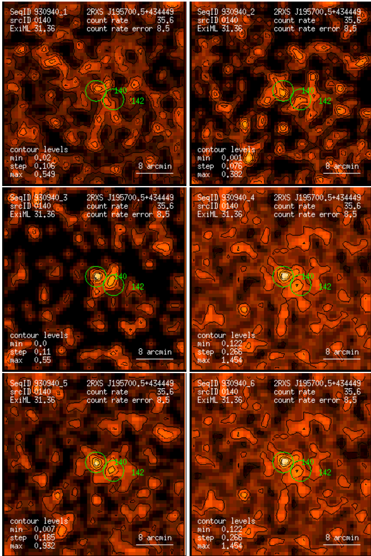
Figure 140: RASS 930940: detection 0140: band rate images, Gaussian filter: (1) PSPC channels 11 – 41, (2) 52 – 90, (3) 91 – 201, (4) 11 – 235, (5) 52 – 201, (6) 11 – 201. Broad band rates in counts/ks. Band rate contour levels in counts/ks/arcmin 2 .
