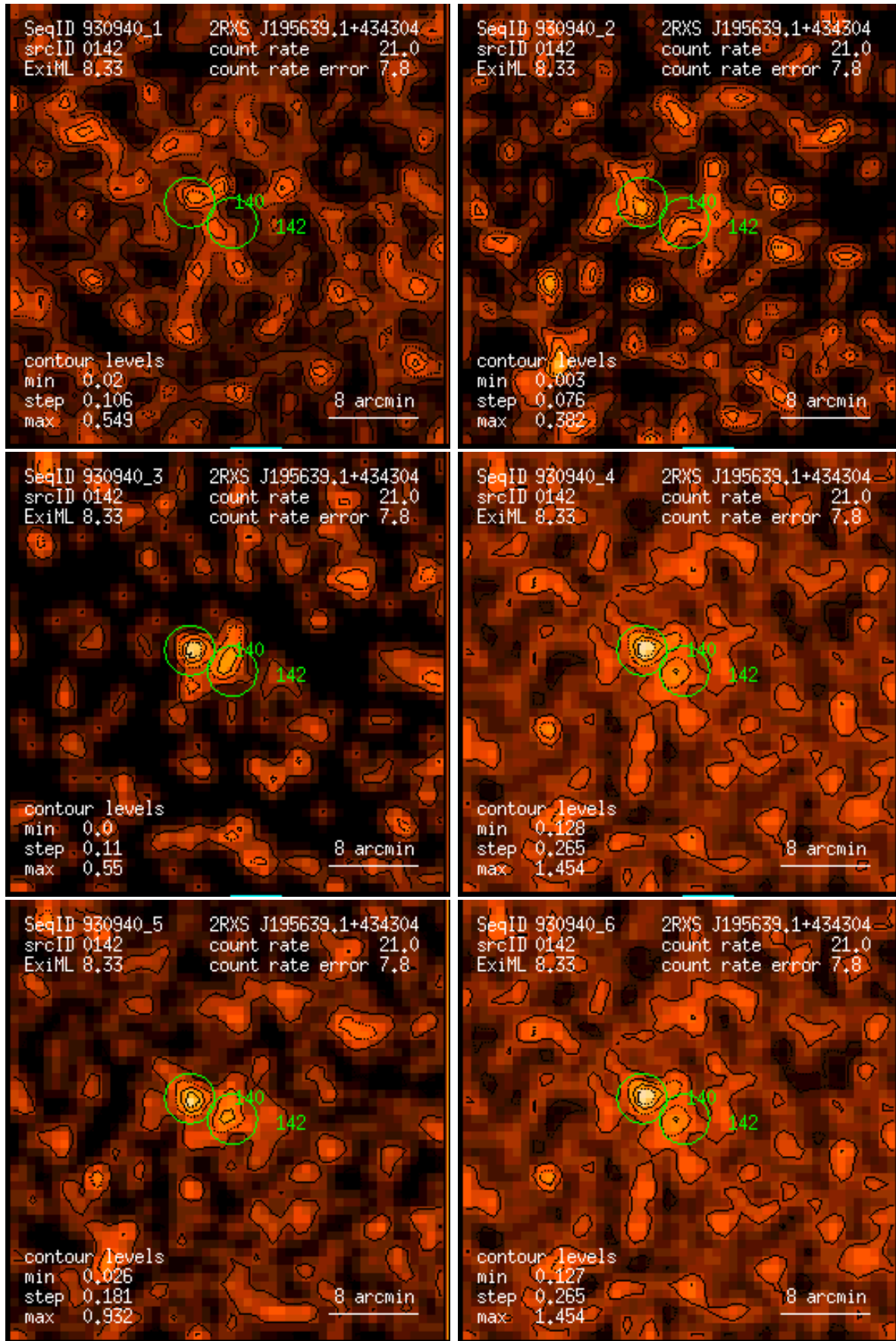
Figure 142: RASS 930940: detection 0142: band rate images, Gaussian filter: (1) PSPC channels 11 – 41, (2) 52 – 90, (3) 91 – 201, (4) 11 – 235, (5) 52 – 201, (6) 11 – 201. Broad band rates in counts/ks. Band rate contour levels in counts/ks/arcmin 2 .
