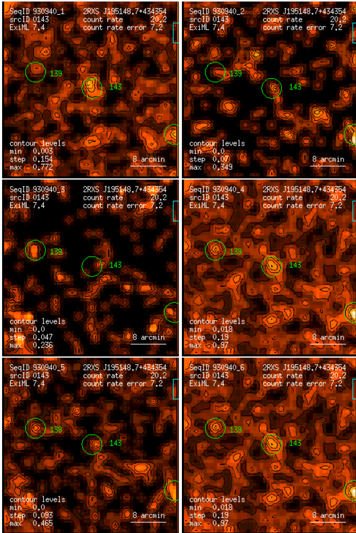
Figure 143: RASS 930940: detection 0143: band rate images, Gaussian filter: (1) PSPC channels 11 – 41, (2) 52 – 90, (3) 91 – 201, (4) 11 – 235, (5) 52 – 201, (6) 11 – 201. Broad band rates in counts/ks. Band rate contour levels in counts/ks/arcmin 2 .
