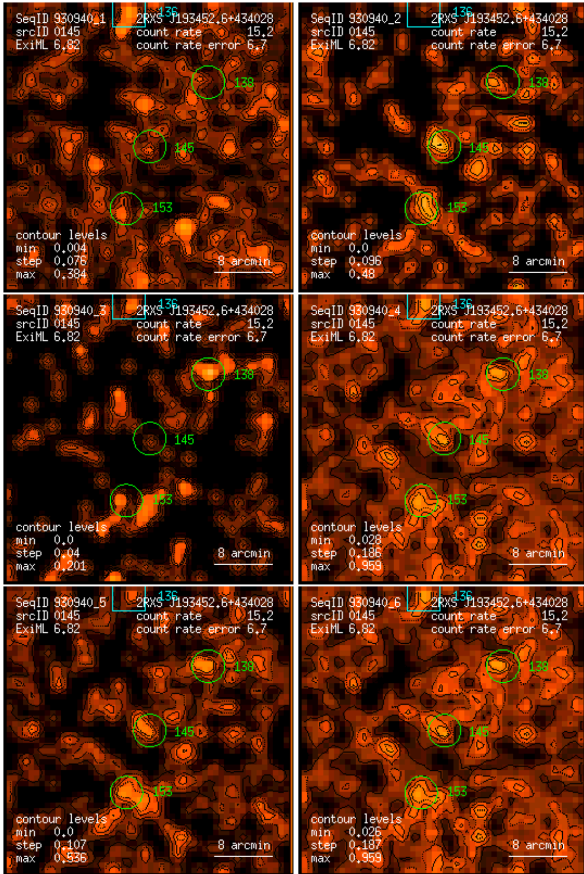
Figure 145: RASS 930940: detection 0145: band rate images, Gaussian filter: (1) PSPC channels 11 – 41, (2) 52 – 90, (3) 91 – 201, (4) 11 – 235, (5) 52 – 201, (6) 11 – 201. Broad band rates in counts/ks. Band rate contour levels in counts/ks/arcmin 2 .
