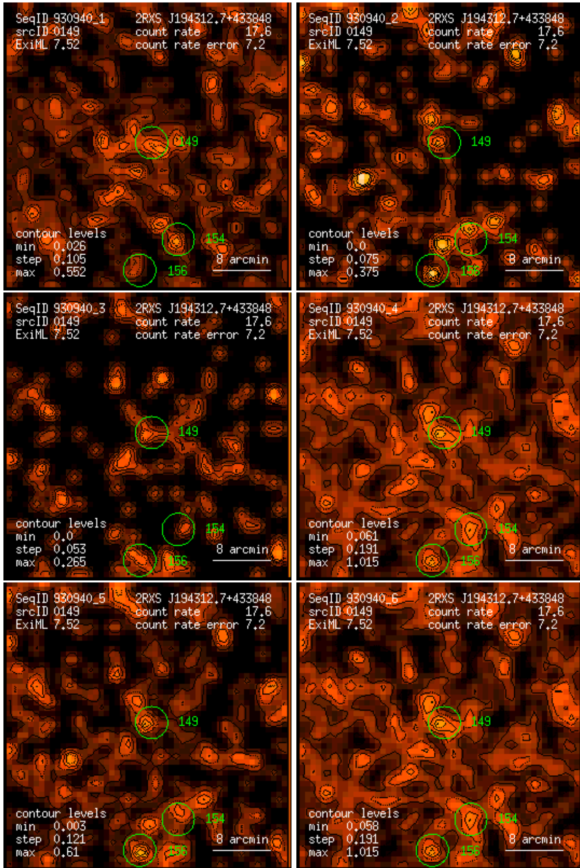
Figure 149: RASS 930940: detection 0149: band rate images, Gaussian filter: (1) PSPC channels 11 – 41, (2) 52 – 90, (3) 91 – 201, (4) 11 – 235, (5) 52 – 201, (6) 11 – 201. Broad band rates in counts/ks. Band rate contour levels in counts/ks/arcmin 2 .
