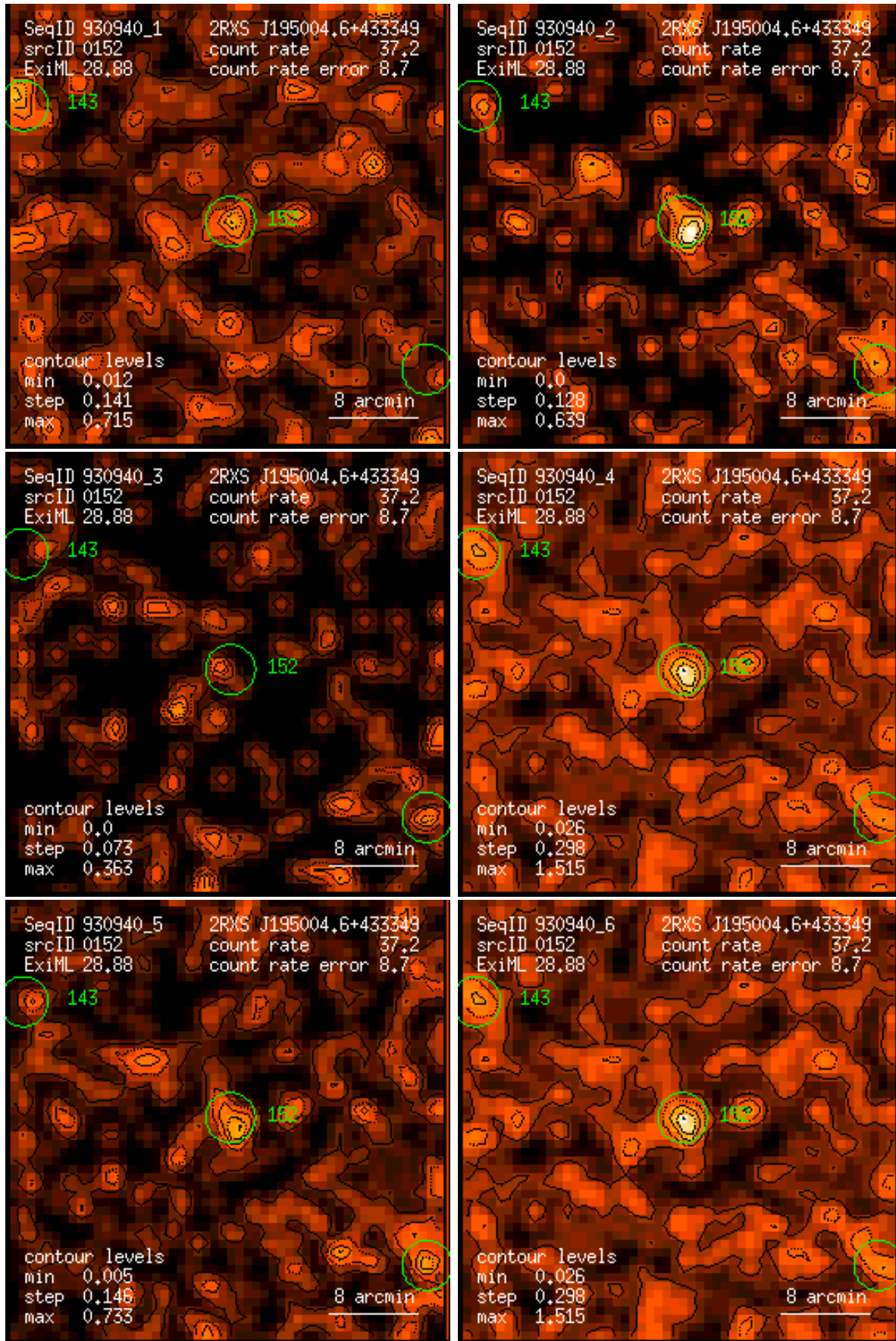
Figure 152: RASS 930940: detection 0152: band rate images, Gaussian filter: (1) PSPC channels 11 – 41, (2) 52 – 90, (3) 91 – 201, (4) 11 – 235, (5) 52 – 201, (6) 11 – 201. Broad band rates in counts/ks. Band rate contour levels in counts/ks/arcmin 2 .
