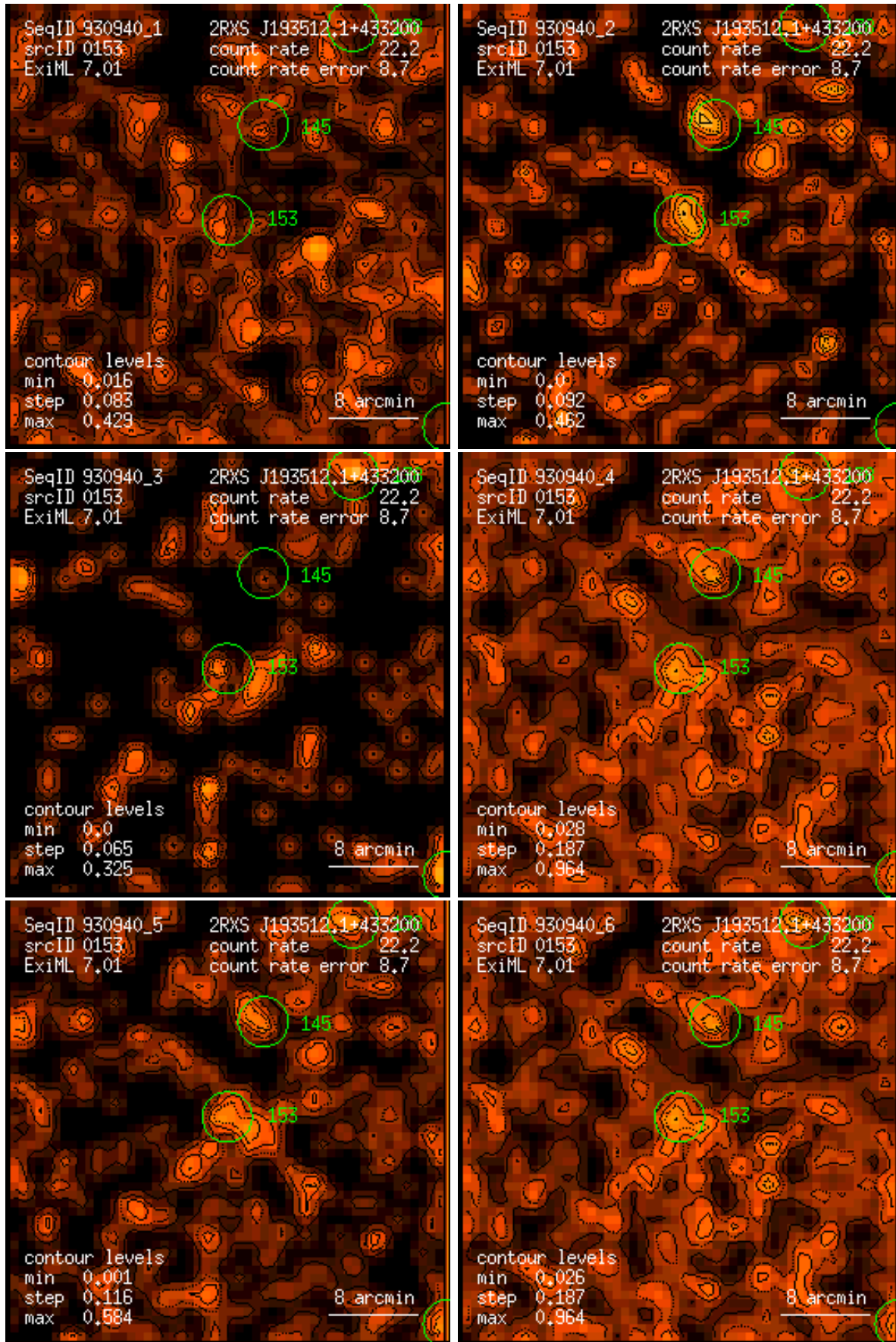
Figure 153: RASS 930940: detection 0153: band rate images, Gaussian filter: (1) PSPC channels 11 – 41, (2) 52 – 90, (3) 91 – 201, (4) 11 – 235, (5) 52 – 201, (6) 11 – 201. Broad band rates in counts/ks. Band rate contour levels in counts/ks/arcmin 2 .
