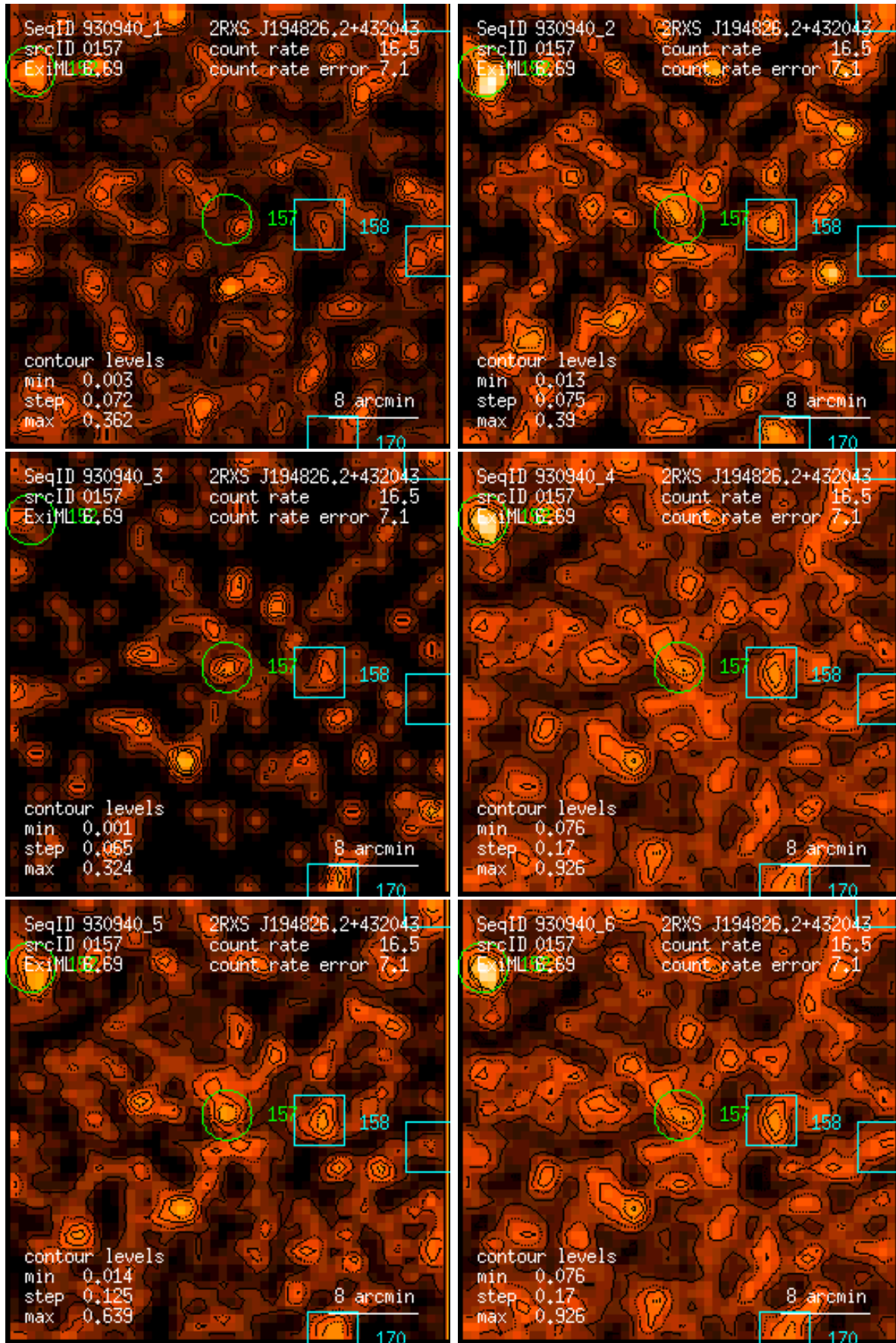
Figure 157: RASS 930940: detection 0157: band rate images, Gaussian filter: (1) PSPC channels 11 – 41, (2) 52 – 90, (3) 91 – 201, (4) 11 – 235, (5) 52 – 201, (6) 11 – 201. Broad band rates in counts/ks. Band rate contour levels in counts/ks/arcmin 2 .
