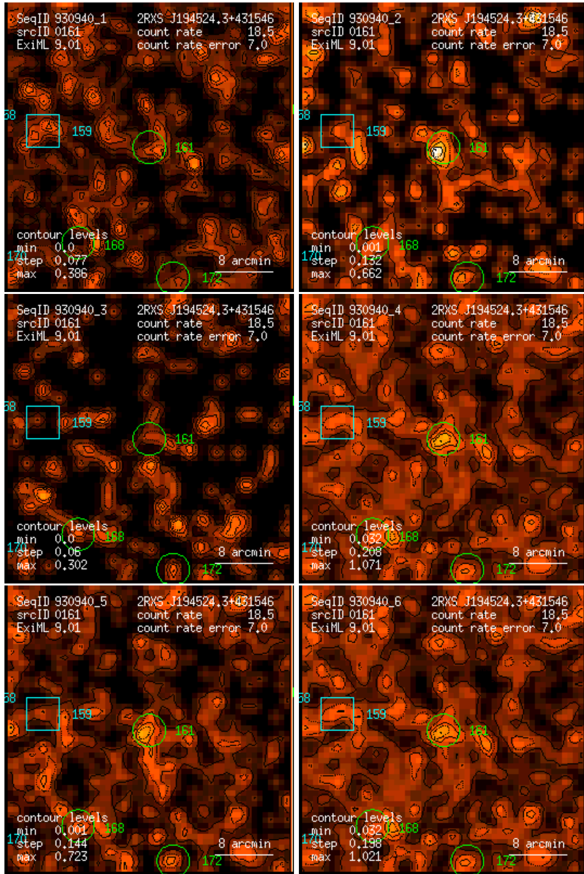
Figure 161: RASS 930940: detection 0161: band rate images, Gaussian filter: (1) PSPC channels 11 – 41, (2) 52 – 90, (3) 91 – 201, (4) 11 – 235, (5) 52 – 201, (6) 11 – 201. Broad band rates in counts/ks. Band rate contour levels in counts/ks/arcmin 2 .
