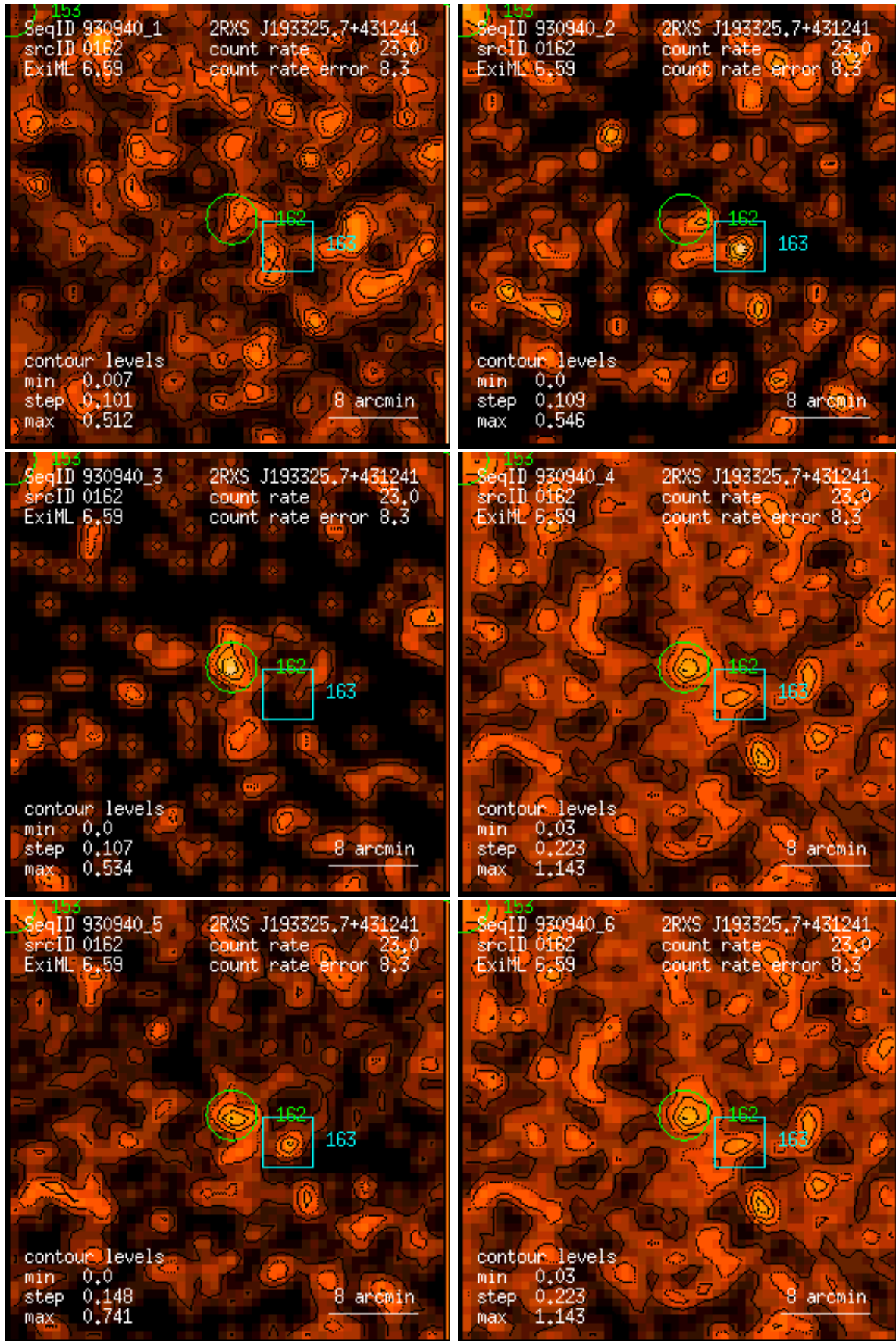
Figure 162: RASS 930940: detection 0162: band rate images, Gaussian filter: (1) PSPC channels 11 – 41, (2) 52 – 90, (3) 91 – 201, (4) 11 – 235, (5) 52 – 201, (6) 11 – 201. Broad band rates in counts/ks. Band rate contour levels in counts/ks/arcmin 2 .
