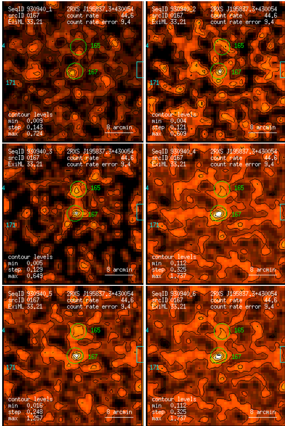
Figure 167: RASS 930940: detection 0167: band rate images, Gaussian filter: (1) PSPC channels 11 – 41, (2) 52 – 90, (3) 91 – 201, (4) 11 – 235, (5) 52 – 201, (6) 11 – 201. Broad band rates in counts/ks. Band rate contour levels in counts/ks/arcmin 2 .
