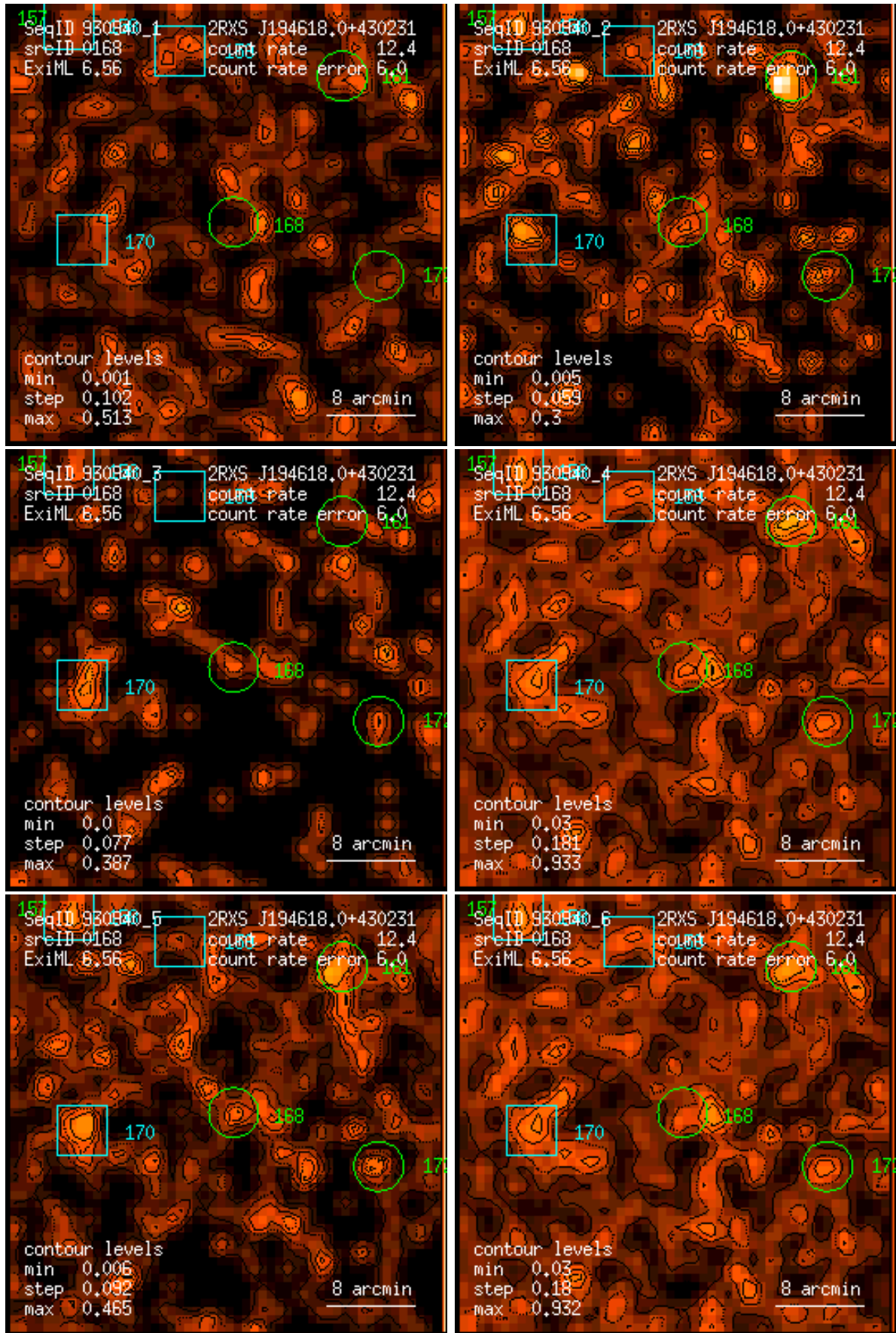
Figure 168: RASS 930940: detection 0168: band rate images, Gaussian filter: (1) PSPC channels 11 – 41, (2) 52 – 90, (3) 91 – 201, (4) 11 – 235, (5) 52 – 201, (6) 11 – 201. Broad band rates in counts/ks. Band rate contour levels in counts/ks/arcmin 2 .
