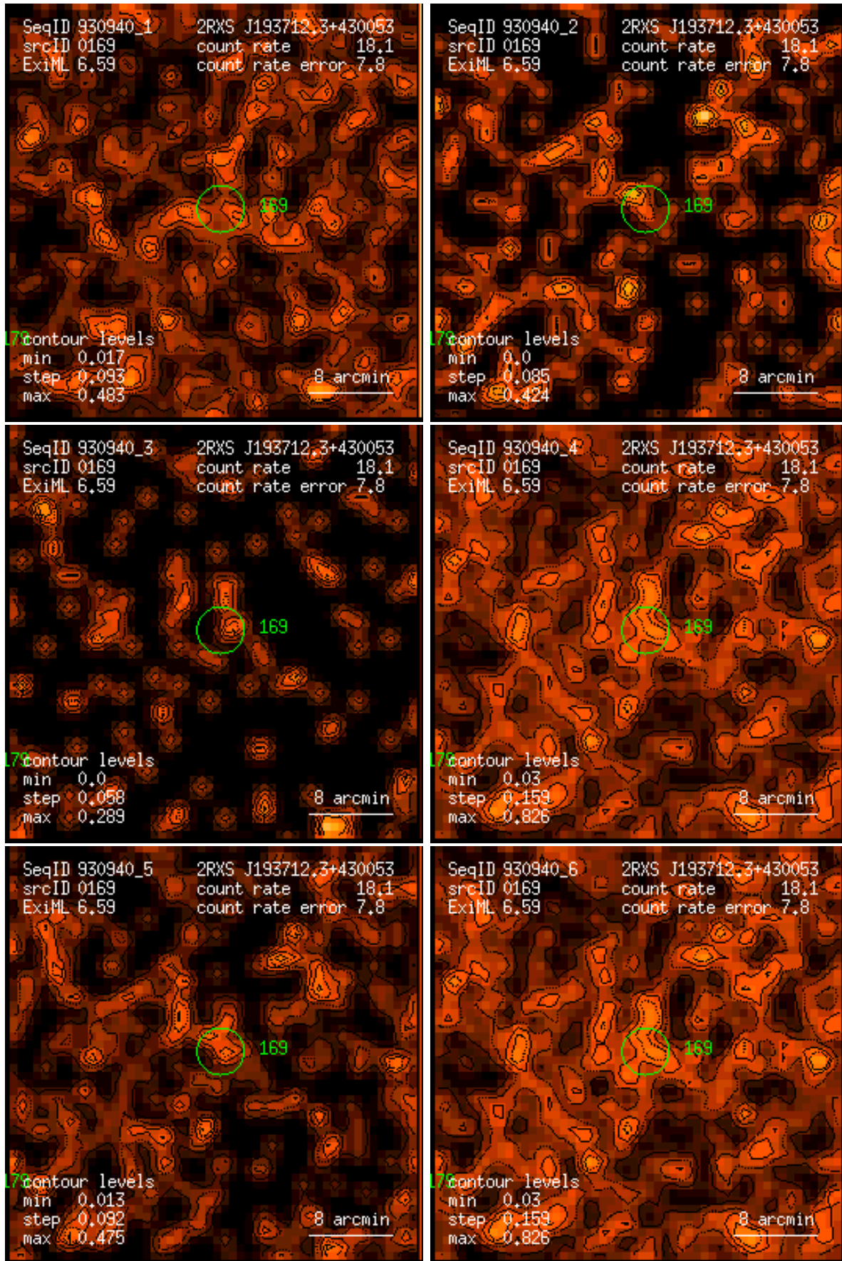
Figure 169: RASS 930940: detection 0169: band rate images, Gaussian filter: (1) PSPC channels 11 – 41, (2) 52 – 90, (3) 91 – 201, (4) 11 – 235, (5) 52 – 201, (6) 11 – 201. Broad band rates in counts/ks. Band rate contour levels in counts/ks/arcmin 2 .
