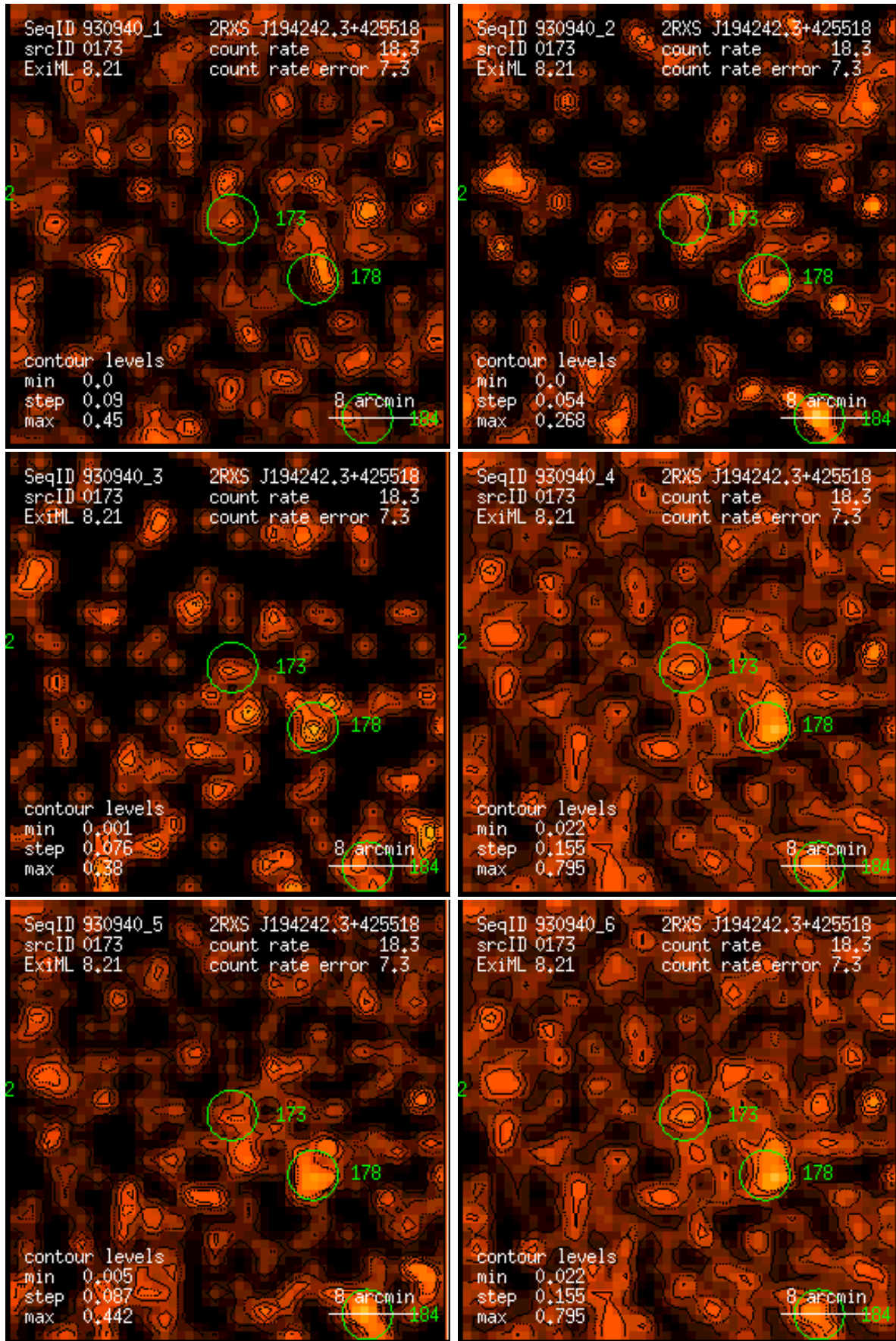
Figure 173: RASS 930940: detection 0173: band rate images, Gaussian filter: (1) PSPC channels 11 – 41, (2) 52 – 90, (3) 91 – 201, (4) 11 – 235, (5) 52 – 201, (6) 11 – 201. Broad band rates in counts/ks. Band rate contour levels in counts/ks/arcmin 2 .
