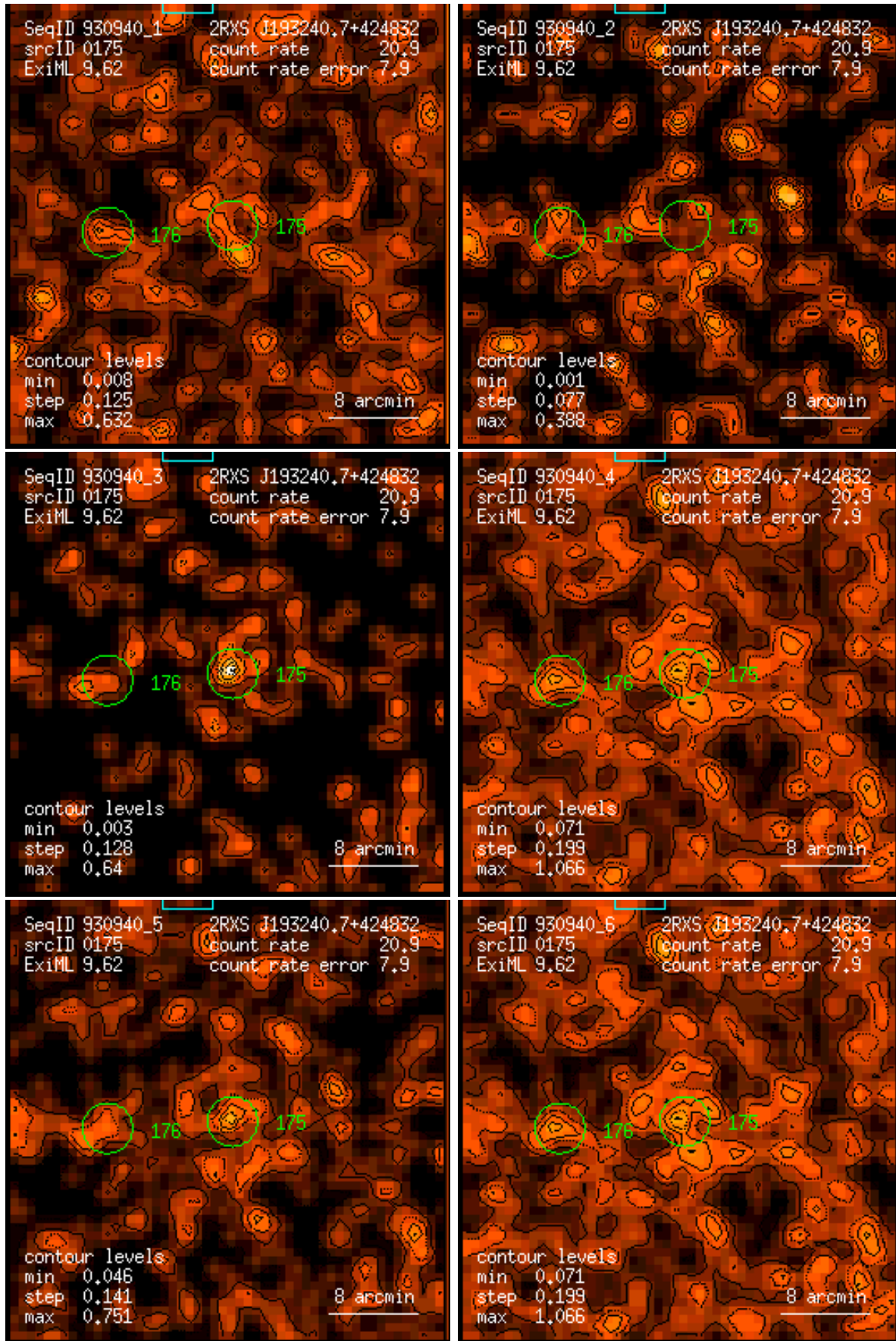
Figure 175: RASS 930940: detection 0175: band rate images, Gaussian filter: (1) PSPC channels 11 – 41, (2) 52 – 90, (3) 91 – 201, (4) 11 – 235, (5) 52 – 201, (6) 11 – 201. Broad band rates in counts/ks. Band rate contour levels in counts/ks/arcmin 2 .
