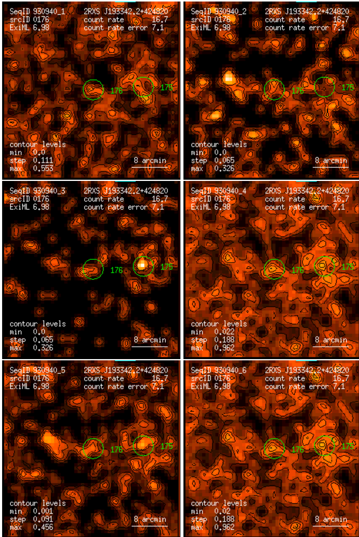
Figure 176: RASS 930940: detection 0176: band rate images, Gaussian filter: (1) PSPC channels 11 – 41, (2) 52 – 90, (3) 91 – 201, (4) 11 – 235, (5) 52 – 201, (6) 11 – 201. Broad band rates in counts/ks. Band rate contour levels in counts/ks/arcmin 2 .
