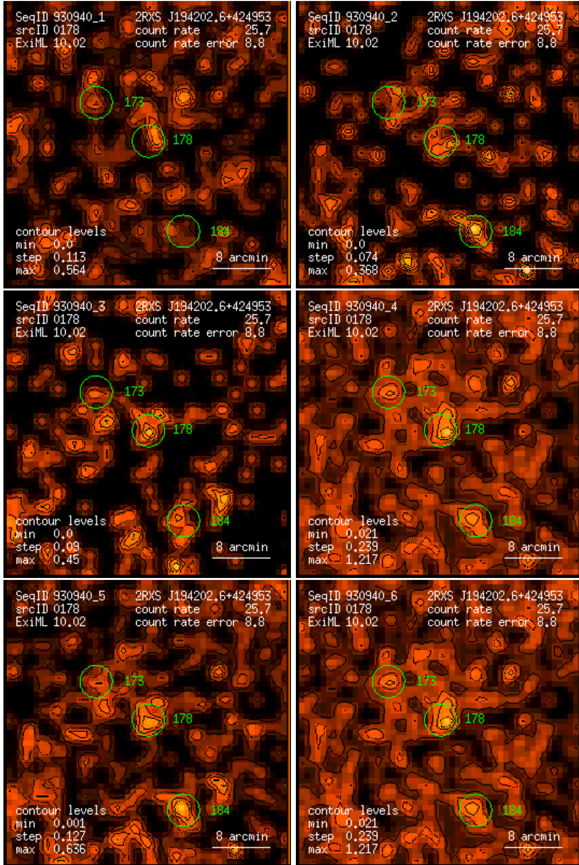
Figure 178: RASS 930940: detection 0178: band rate images, Gaussian filter: (1) PSPC channels 11 – 41, (2) 52 – 90, (3) 91 – 201, (4) 11 – 235, (5) 52 – 201, (6) 11 – 201. Broad band rates in counts/ks. Band rate contour levels in counts/ks/arcmin 2 .
