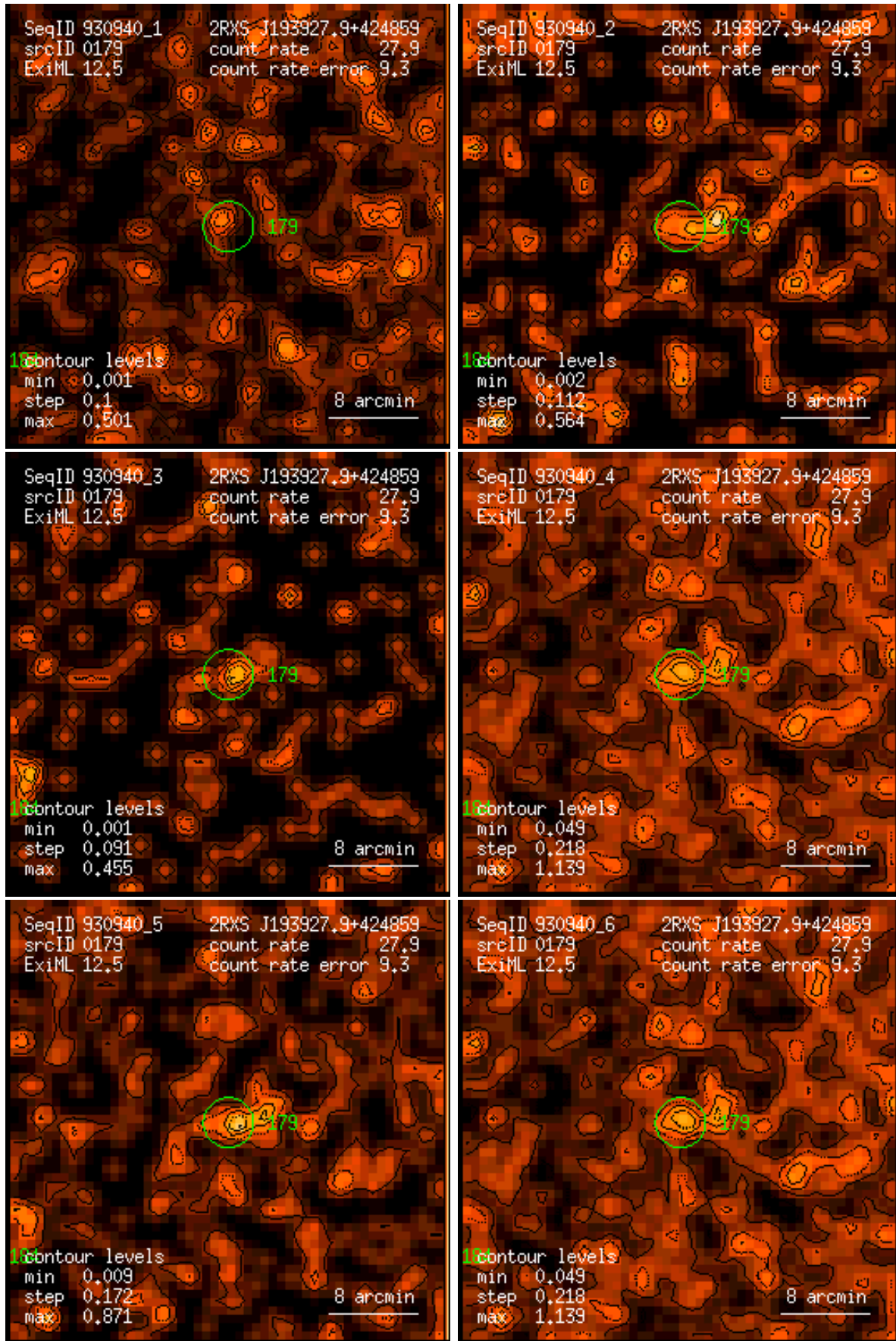
Figure 179: RASS 930940: detection 0179: band rate images, Gaussian filter: (1) PSPC channels 11 – 41, (2) 52 – 90, (3) 91 – 201, (4) 11 – 235, (5) 52 – 201, (6) 11 – 201. Broad band rates in counts/ks. Band rate contour levels in counts/ks/arcmin 2 .
