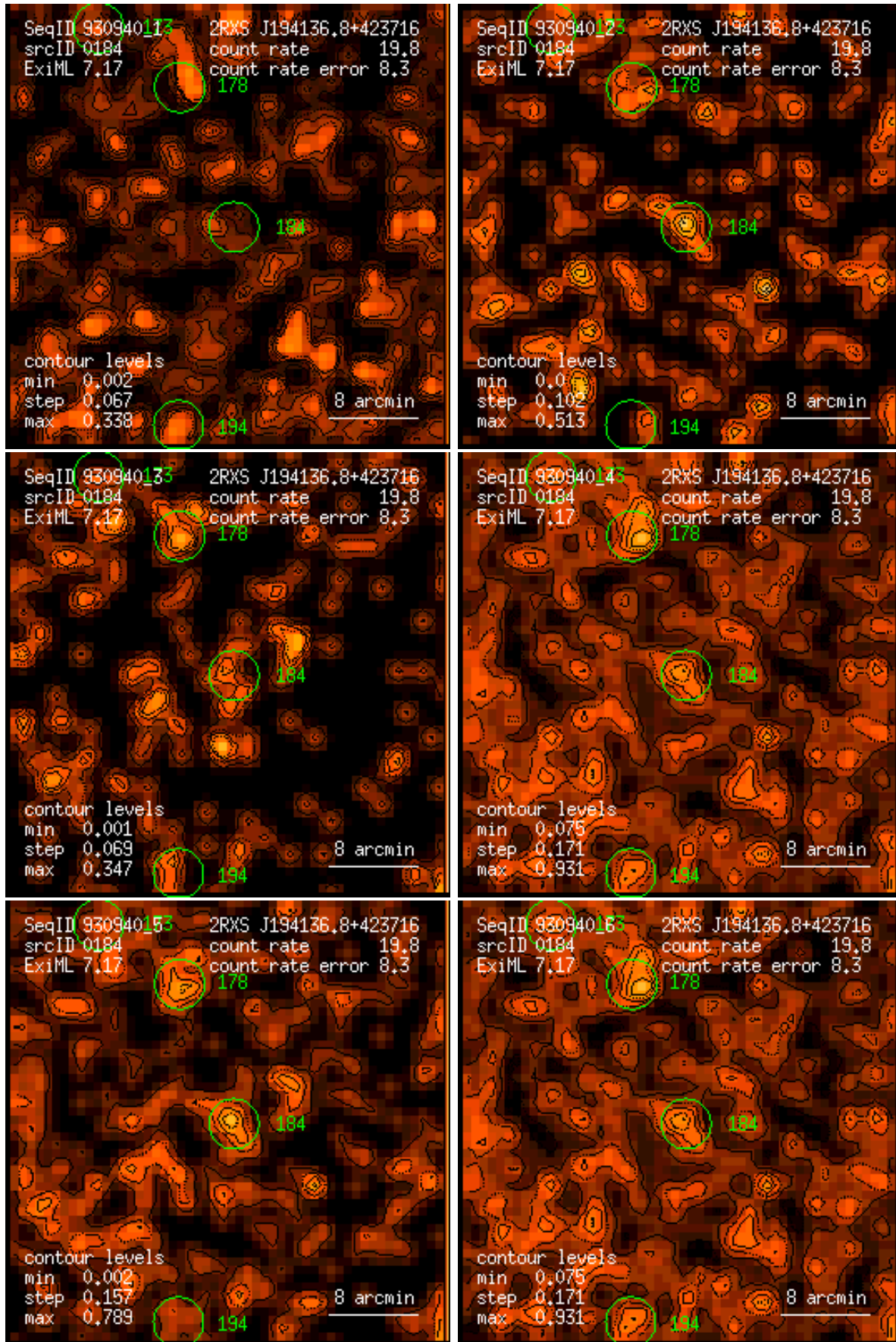
Figure 184: RASS 930940: detection 0184: band rate images, Gaussian filter: (1) PSPC channels 11 – 41, (2) 52 – 90, (3) 91 – 201, (4) 11 – 235, (5) 52 – 201, (6) 11 – 201. Broad band rates in counts/ks. Band rate contour levels in counts/ks/arcmin 2 .
