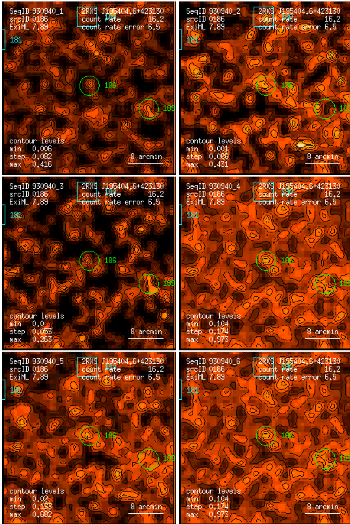
Figure 186: RASS 930940: detection 0186: band rate images, Gaussian filter: (1) PSPC channels 11 – 41, (2) 52 – 90, (3) 91 – 201, (4) 11 – 235, (5) 52 – 201, (6) 11 – 201. Broad band rates in counts/ks. Band rate contour levels in counts/ks/arcmin 2 .
