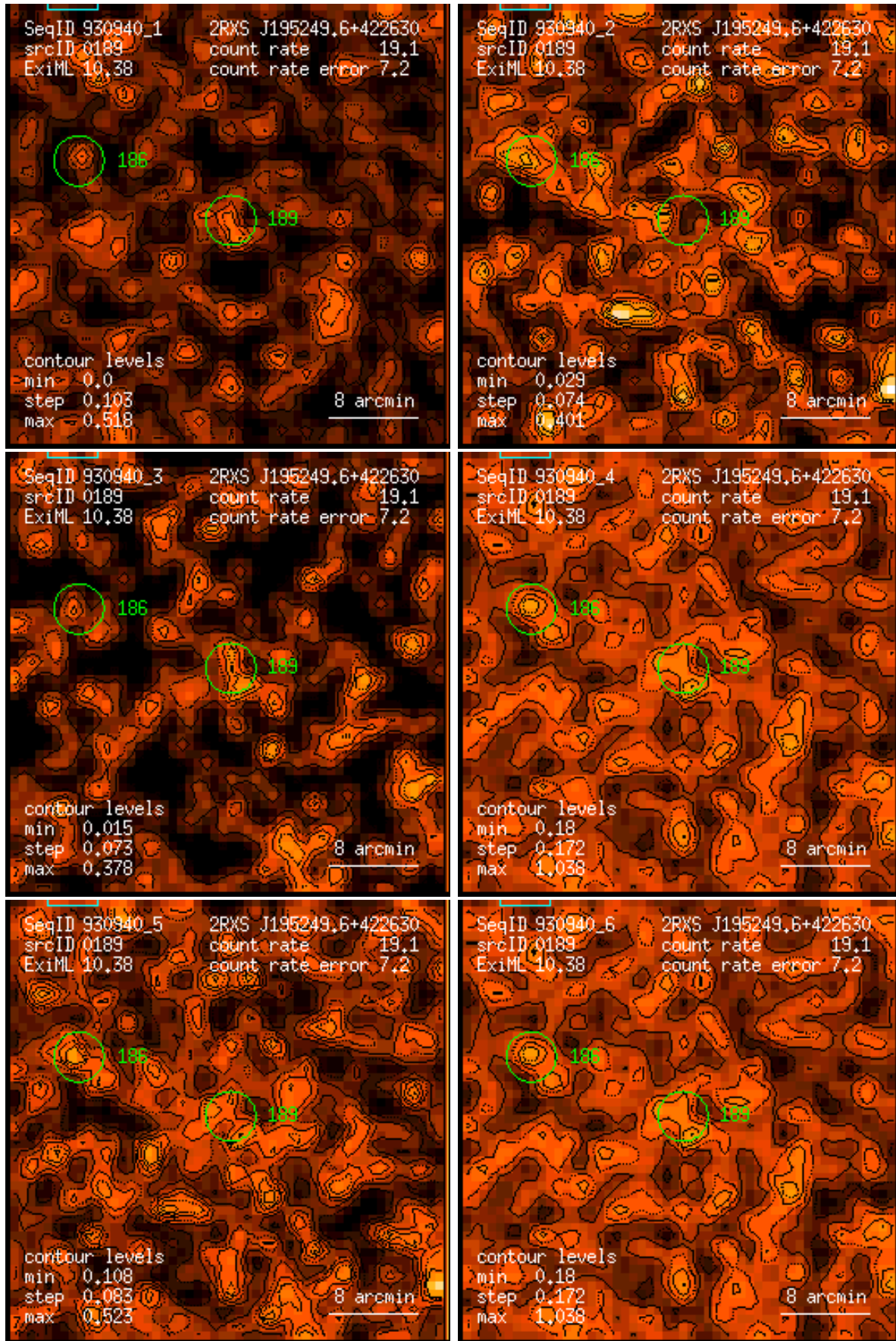
Figure 189: RASS 930940: detection 0189: band rate images, Gaussian filter: (1) PSPC channels 11 – 41, (2) 52 – 90, (3) 91 – 201, (4) 11 – 235, (5) 52 – 201, (6) 11 – 201. Broad band rates in counts/ks. Band rate contour levels in counts/ks/arcmin 2 .
