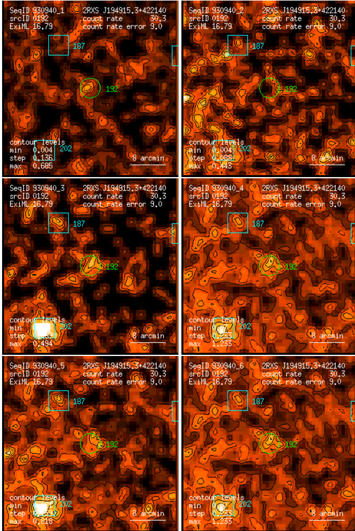
Figure 192: RASS 930940: detection 0192: band rate images, Gaussian filter: (1) PSPC channels 11 – 41, (2) 52 – 90, (3) 91 – 201, (4) 11 – 235, (5) 52 – 201, (6) 11 – 201. Broad band rates in counts/ks. Band rate contour levels in counts/ks/arcmin 2 .
