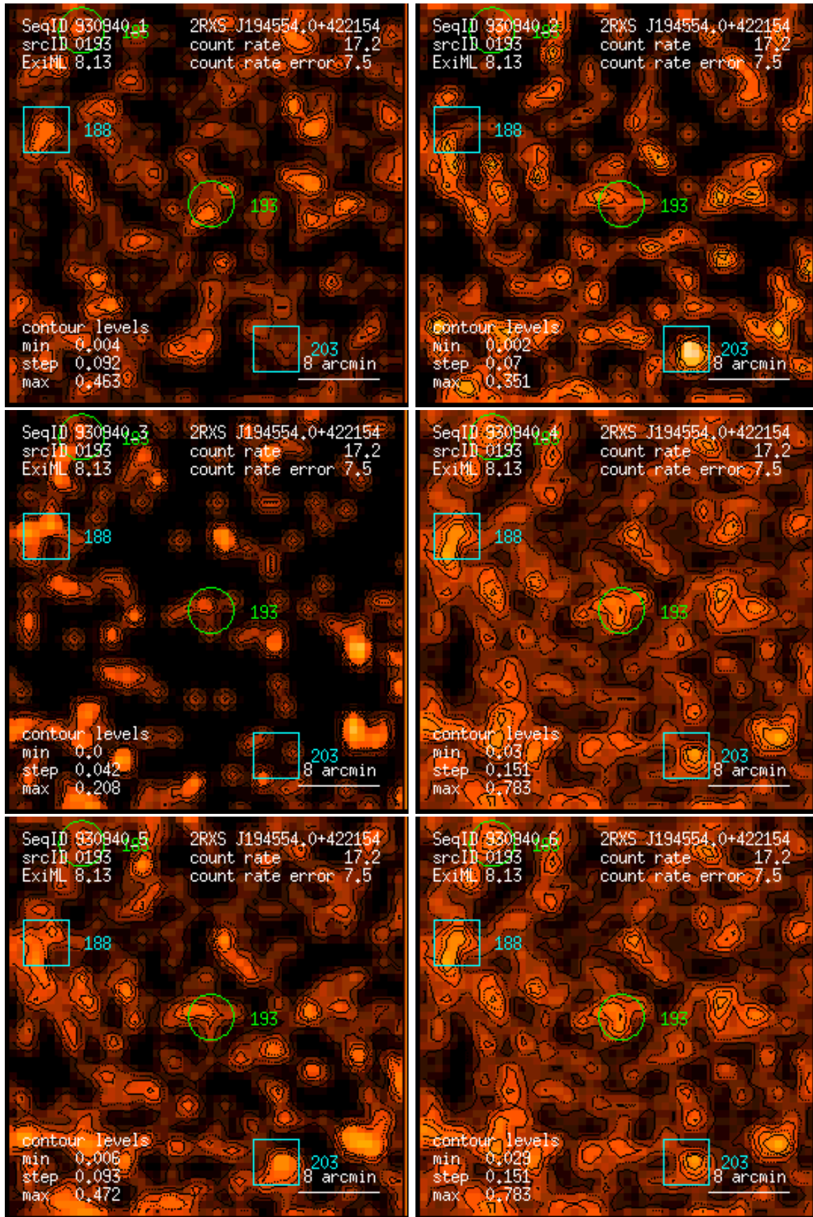
Figure 193: RASS 930940: detection 0193: band rate images, Gaussian filter: (1) PSPC channels 11 – 41, (2) 52 – 90, (3) 91 – 201, (4) 11 – 235, (5) 52 – 201, (6) 11 – 201. Broad band rates in counts/ks. Band rate contour levels in counts/ks/arcmin 2 .
