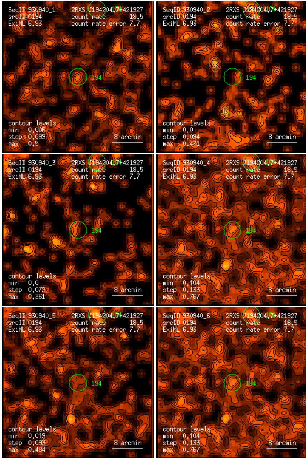
Figure 194: RASS 930940: detection 0194: band rate images, Gaussian filter: (1) PSPC channels 11 – 41, (2) 52 – 90, (3) 91 – 201, (4) 11 – 235, (5) 52 – 201, (6) 11 – 201. Broad band rates in counts/ks. Band rate contour levels in counts/ks/arcmin 2 .
