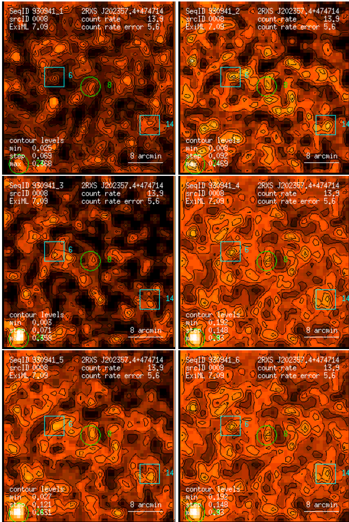
Figure 8: RASS 930941: detection 0008: band rate images, Gaussian filter: (1) PSPC channels 11 – 41, (2) 52 – 90, (3) 91 – 201, (4) 11 – 235, (5) 52 – 201, (6) 11 – 201. Broad band rates in counts/ks. Band rate contour levels in counts/ks/arcmin 2 .
