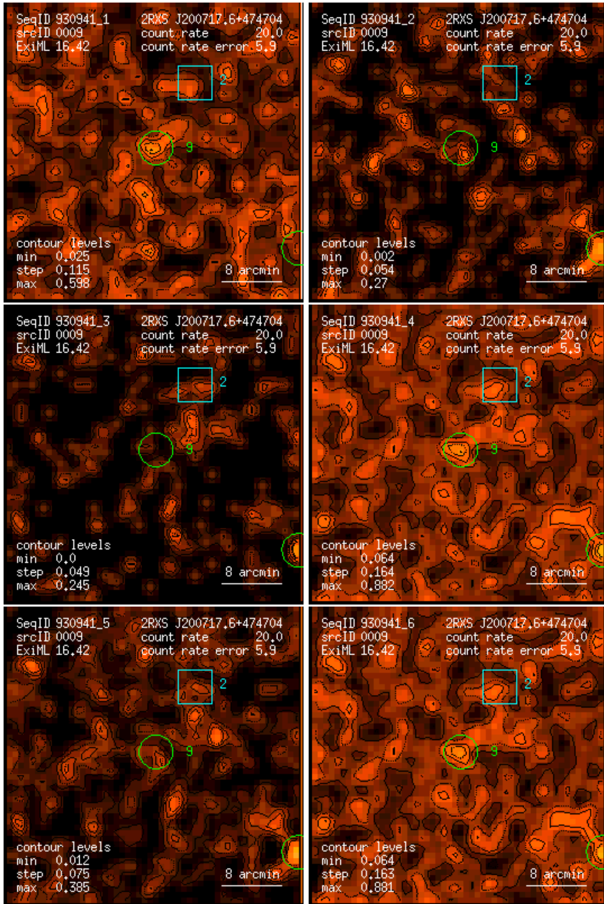
Figure 9: RASS 930941: detection 0009: band rate images, Gaussian filter: (1) PSPC channels 11 – 41, (2) 52 – 90, (3) 91 – 201, (4) 11 – 235, (5) 52 – 201, (6) 11 – 201. Broad band rates in counts/ks. Band rate contour levels in counts/ks/arcmin 2 .
