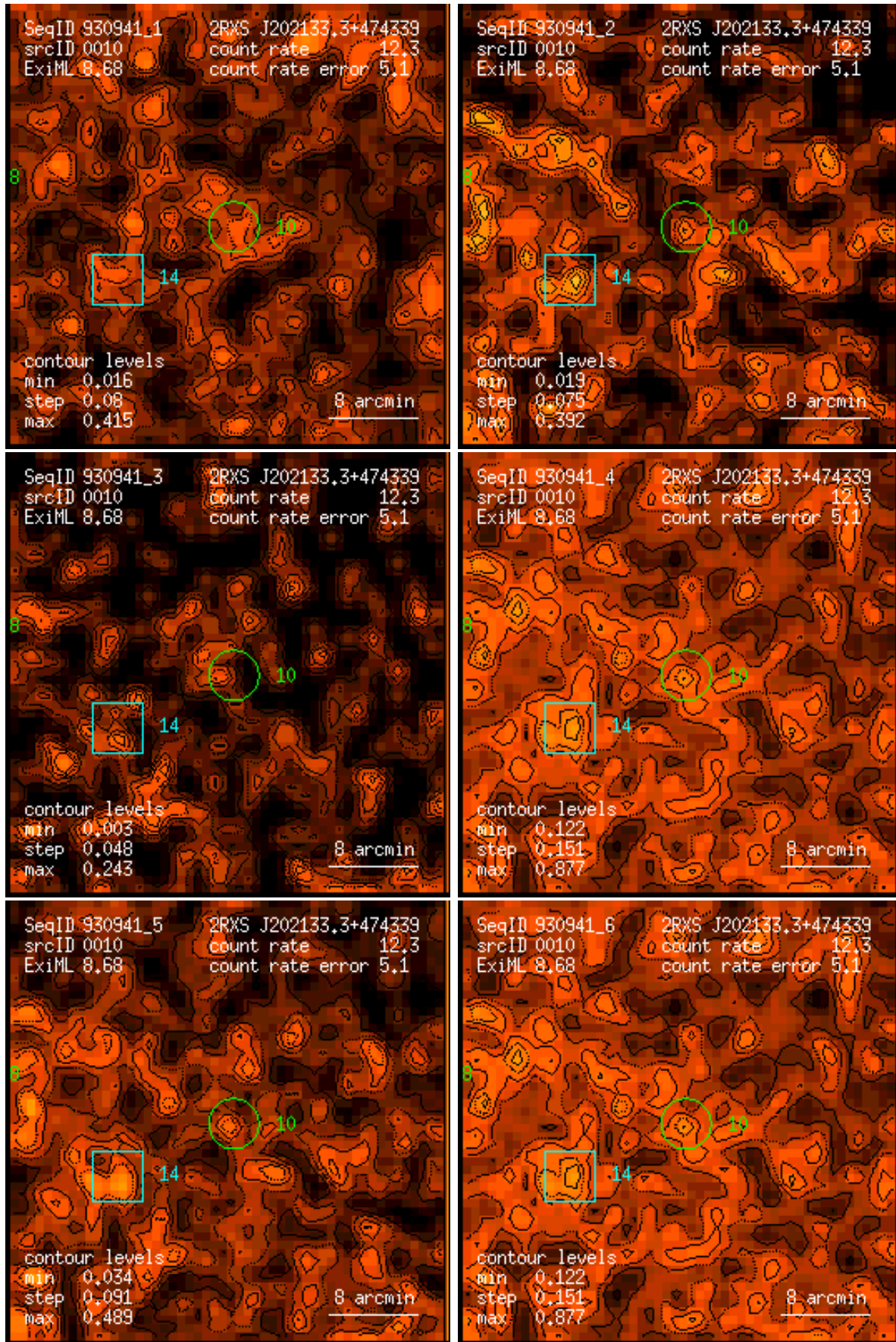
Figure 10: RASS 930941: detection 0010: band rate images, Gaussian filter: (1) PSPC channels 11 – 41, (2) 52 – 90, (3) 91 – 201, (4) 11 – 235, (5) 52 – 201, (6) 11 – 201. Broad band rates in counts/ks. Band rate contour levels in counts/ks/arcmin 2 .
