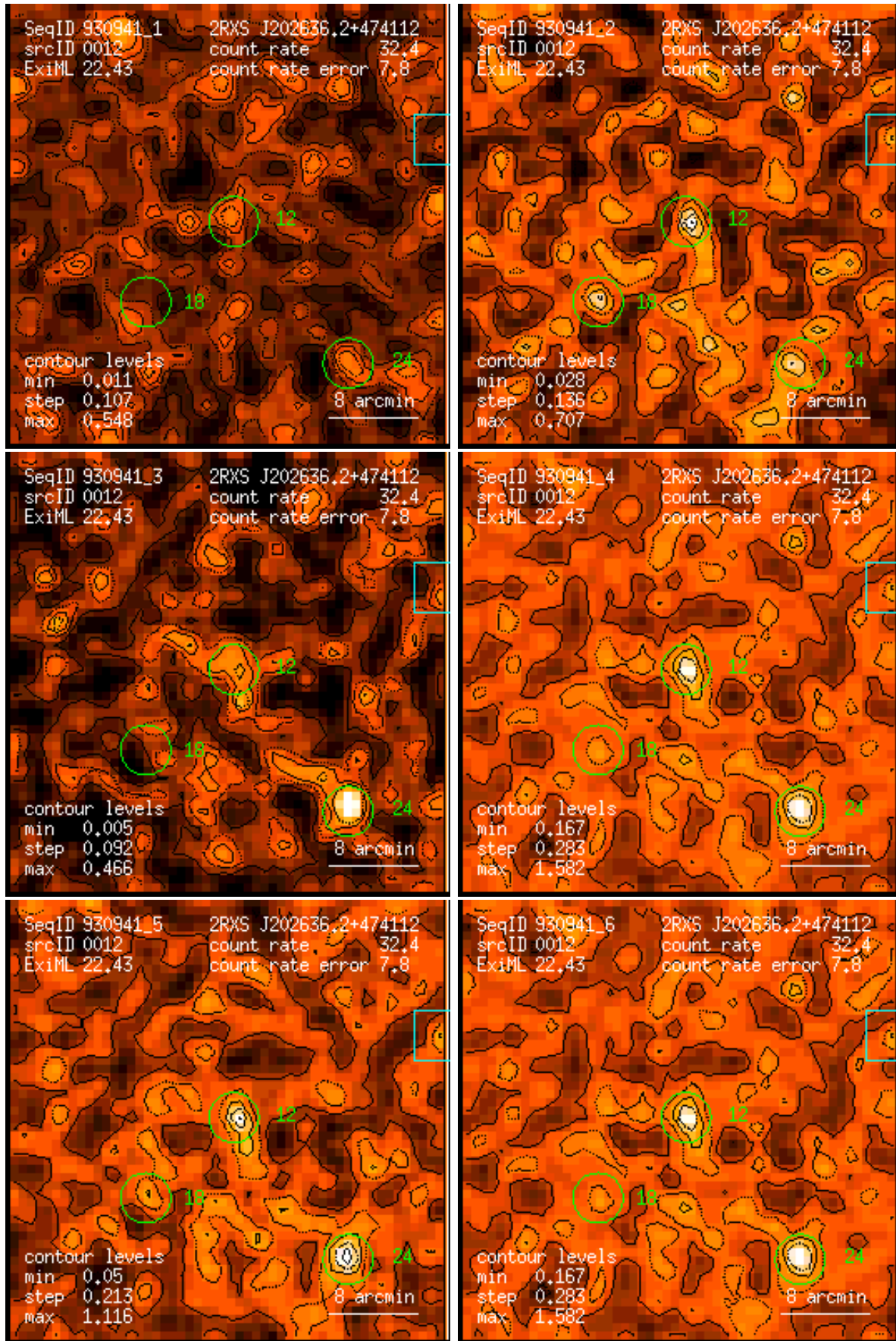
Figure 12: RASS 930941: detection 0012: band rate images, Gaussian filter: (1) PSPC channels 11 – 41, (2) 52 – 90, (3) 91 – 201, (4) 11 – 235, (5) 52 – 201, (6) 11 – 201. Broad band rates in counts/ks. Band rate contour levels in counts/ks/arcmin 2 .
