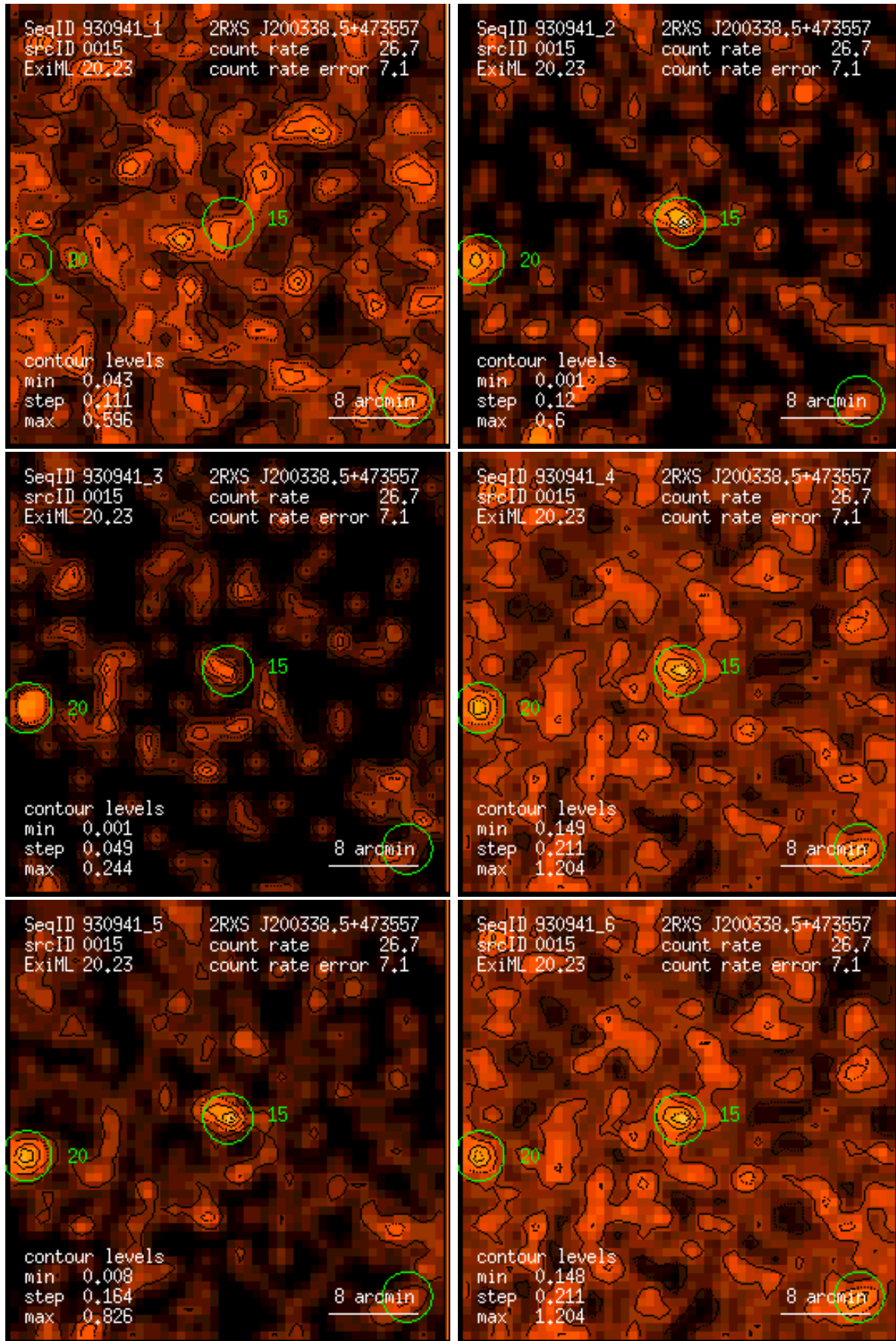
Figure 15: RASS 930941: detection 0015: band rate images, Gaussian filter: (1) PSPC channels 11 – 41, (2) 52 – 90, (3) 91 – 201, (4) 11 – 235, (5) 52 – 201, (6) 11 – 201. Broad band rates in counts/ks. Band rate contour levels in counts/ks/arcmin 2 .
