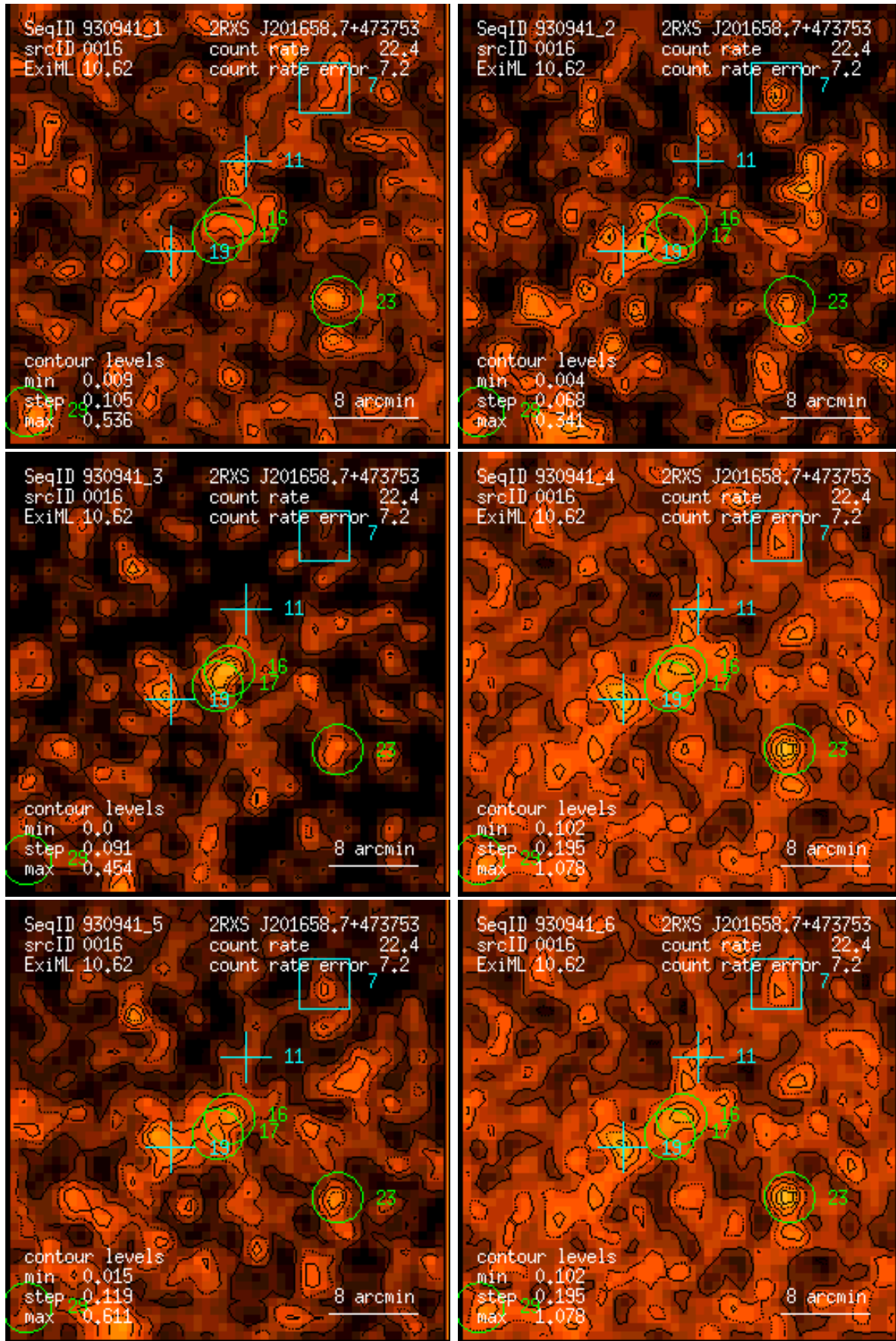
Figure 16: RASS 930941: detection 0016: band rate images, Gaussian filter: (1) PSPC channels 11 – 41, (2) 52 – 90, (3) 91 – 201, (4) 11 – 235, (5) 52 – 201, (6) 11 – 201. Broad band rates in counts/ks. Band rate contour levels in counts/ks/arcmin 2 .
