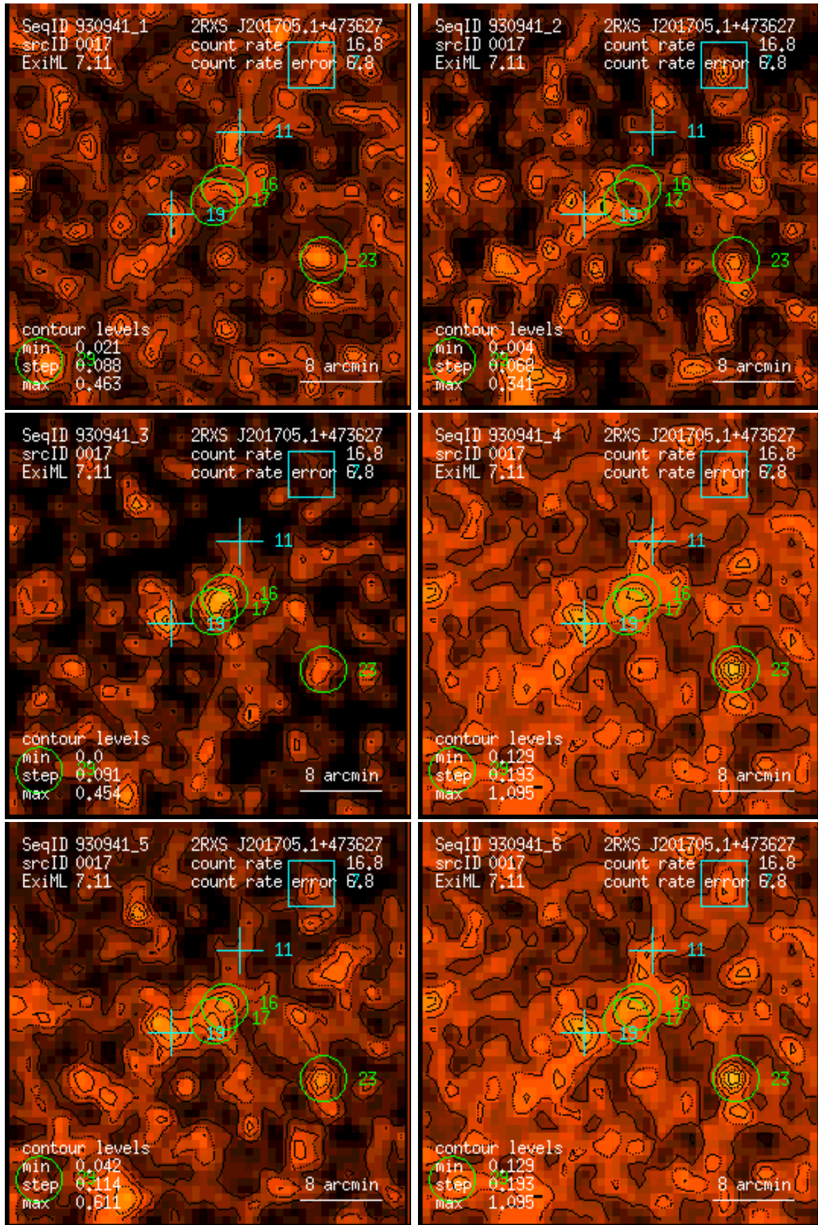
Figure 17: RASS 930941: detection 0017: band rate images, Gaussian filter: (1) PSPC channels 11 – 41, (2) 52 – 90, (3) 91 – 201, (4) 11 – 235, (5) 52 – 201, (6) 11 – 201. Broad band rates in counts/ks. Band rate contour levels in counts/ks/arcmin 2 .
