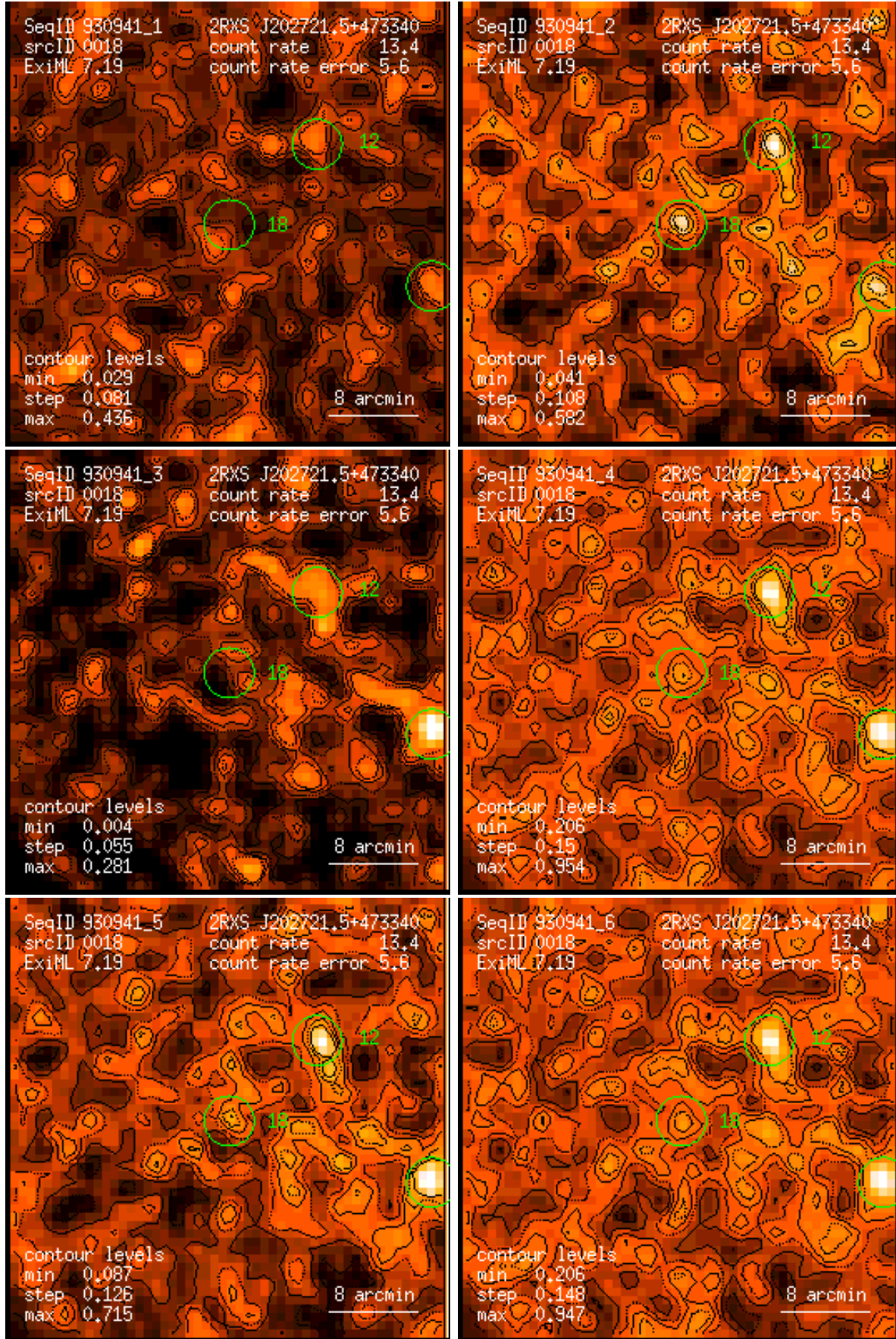
Figure 18: RASS 930941: detection 0018: band rate images, Gaussian filter: (1) PSPC channels 11 – 41, (2) 52 – 90, (3) 91 – 201, (4) 11 – 235, (5) 52 – 201, (6) 11 – 201. Broad band rates in counts/ks. Band rate contour levels in counts/ks/arcmin 2 .
