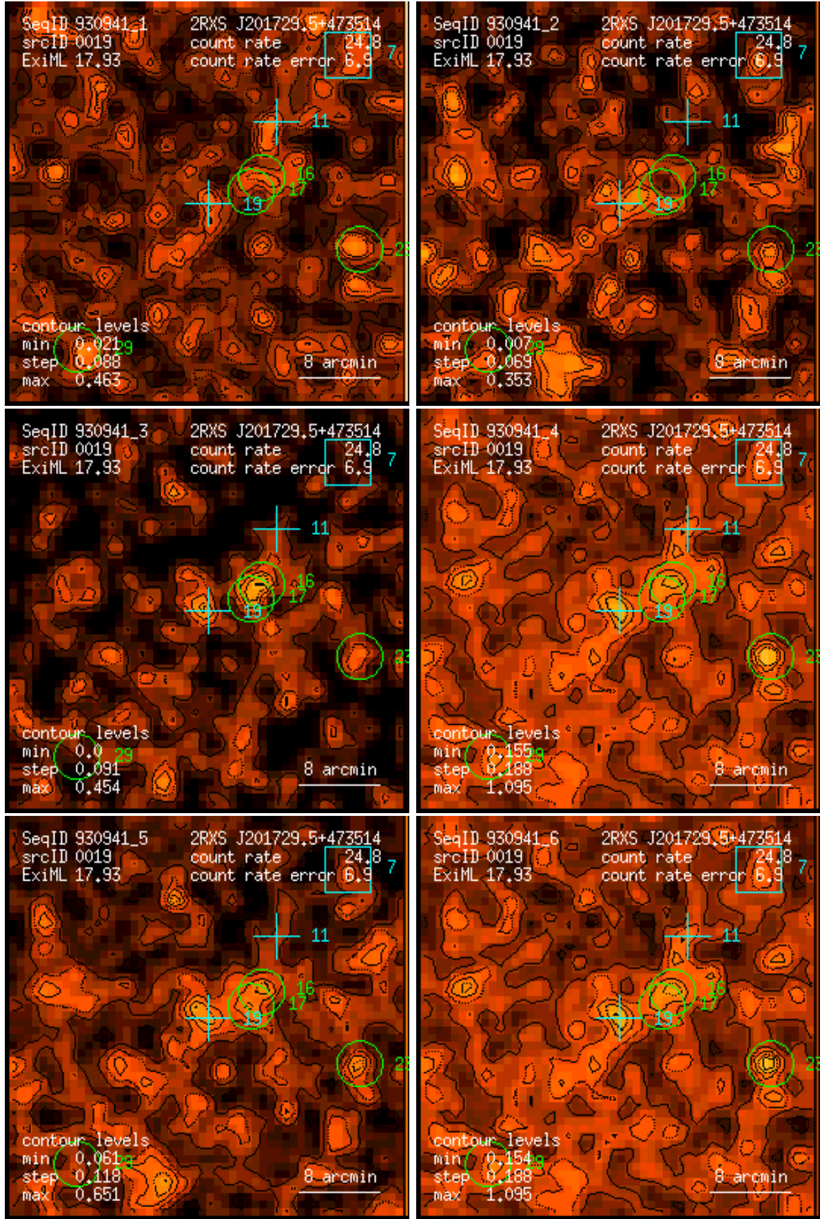
Figure 19: RASS 930941: detection 0019: band rate images, Gaussian filter: (1) PSPC channels 11 – 41, (2) 52 – 90, (3) 91 – 201, (4) 11 – 235, (5) 52 – 201, (6) 11 – 201. Broad band rates in counts/ks. Band rate contour levels in counts/ks/arcmin 2 .
