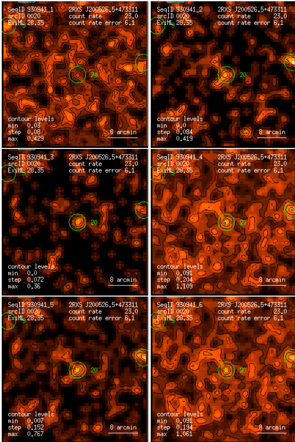
Figure 20: RASS 930941: detection 0020: band rate images, Gaussian filter: (1) PSPC channels 11 – 41, (2) 52 – 90, (3) 91 – 201, (4) 11 – 235, (5) 52 – 201, (6) 11 – 201. Broad band rates in counts/ks. Band rate contour levels in counts/ks/arcmin 2 .
