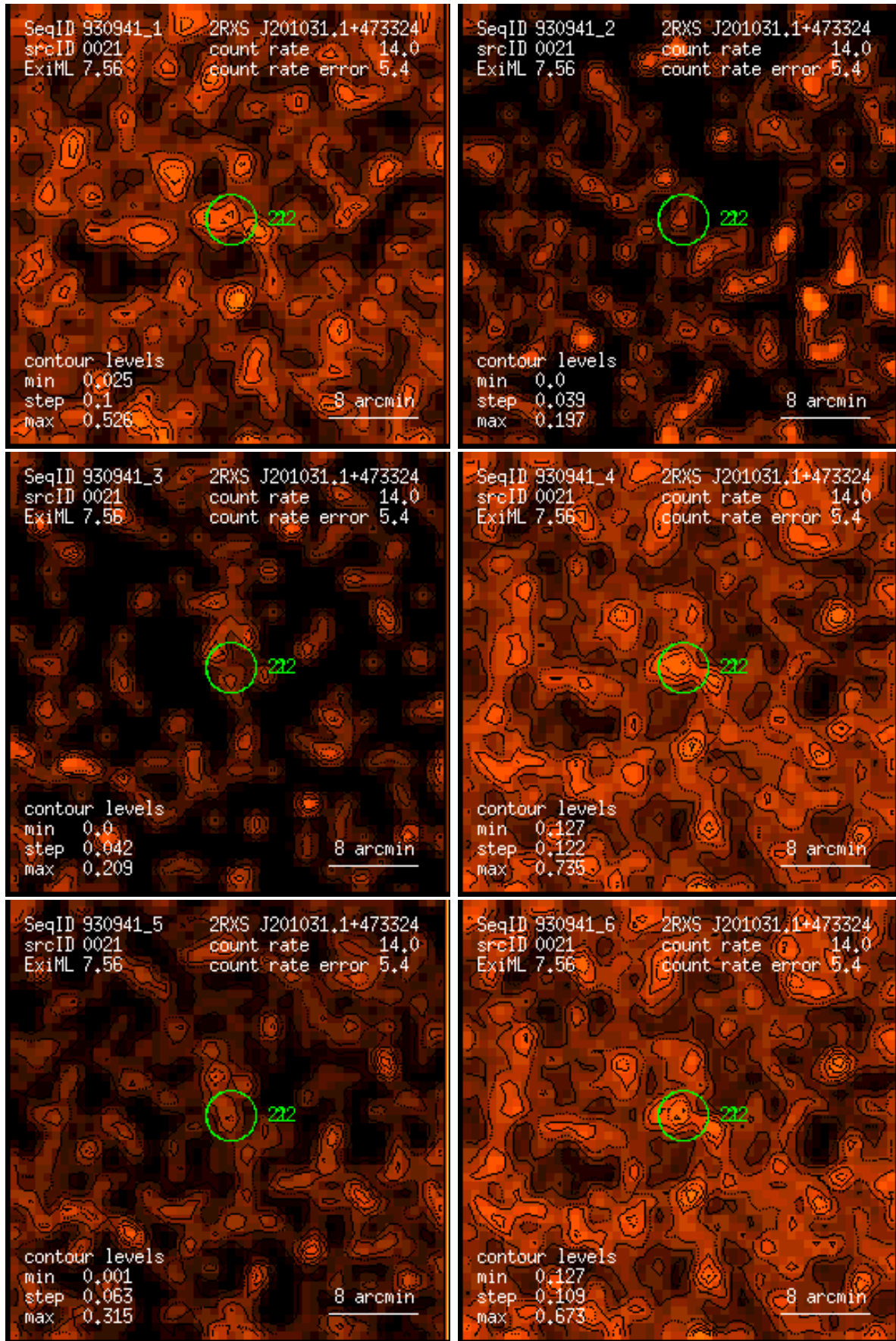
Figure 21: RASS 930941: detection 0021: band rate images, Gaussian filter: (1) PSPC channels 11 – 41, (2) 52 – 90, (3) 91 – 201, (4) 11 – 235, (5) 52 – 201, (6) 11 – 201. Broad band rates in counts/ks. Band rate contour levels in counts/ks/arcmin 2 .
